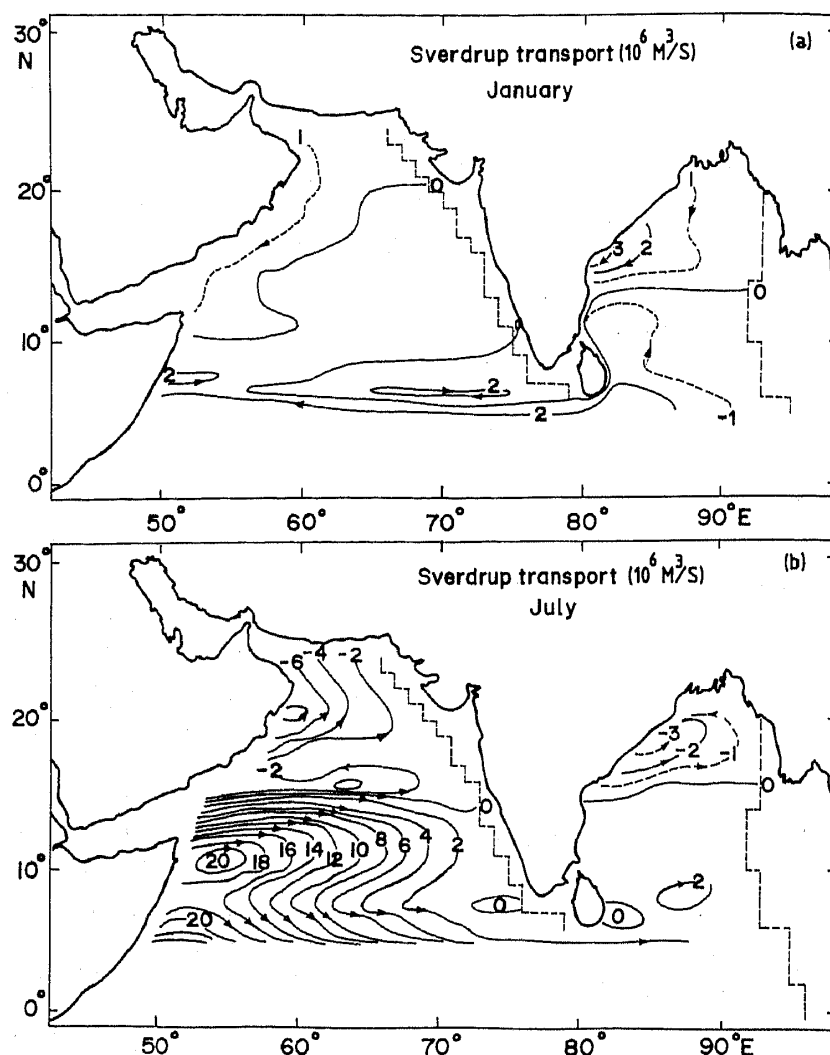
Figure 5. Sverdrup transport: \psi ( 10^6 \text{ m}^3/\text{s} ) in the North Indian Ocean north of 5^\circ\text{N} in (a) January and (b) July. The dashed line in the figure gives the 'eastern boundary' where \psi has been set to zero.
