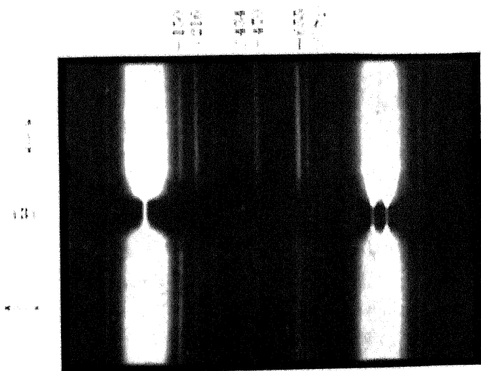
Sulphur in CS 2 - Polarisation.
