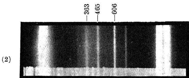
Phosphorus Liquid.
