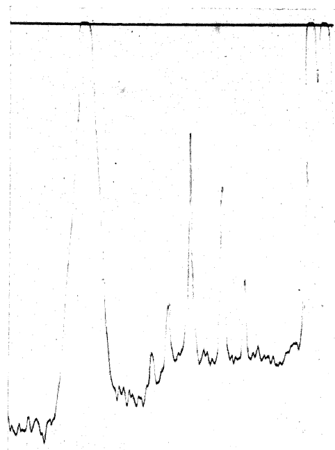
Microphotometric Curves of Fig. (3).
