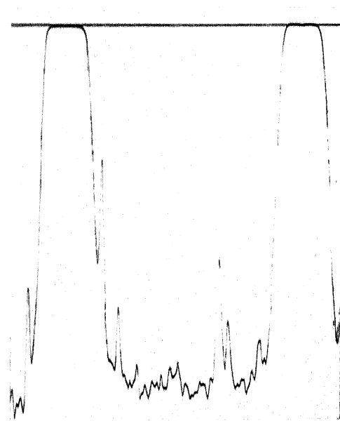
Microphotometric Curves of Fig. (3).
