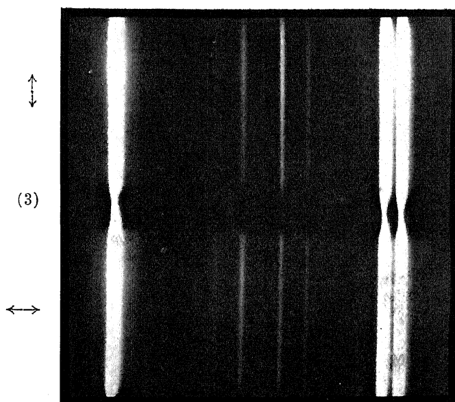
Phosphorus—Polarisation.
