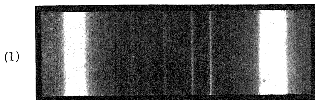
Phosphorus Solid.
