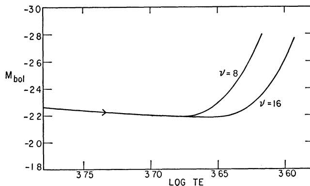
FIG. 7.—Segments of post-main-sequence evolutionary tracks for 5 M_{\odot} , indicating the effect of changing the parameter \nu from 8 to 16. Other parameters have the same values as in Fig. 1.
