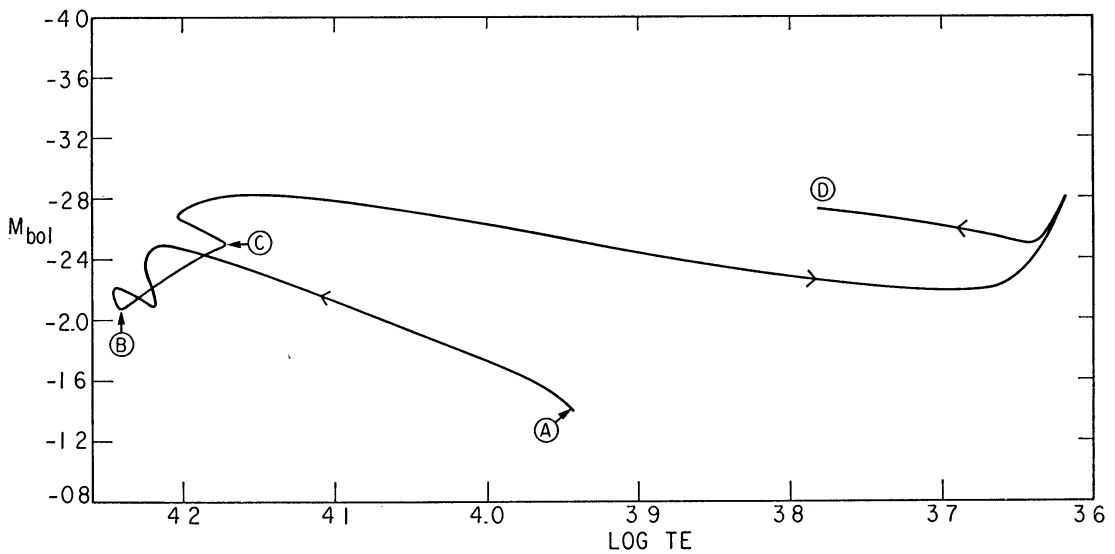
FIG. 1.—The complete evolutionary track in the (\log T_e, M_{bol}) plane computed for 5 M_{\odot} . Indicated points are explained in the text. Appropriate parameters are hydrogen content X = 0.68 ; metal content Z = 0.03 ; l/H = 1.5 ; y = 0.076 ; \beta = 0.5 ; \nu = 8 .
