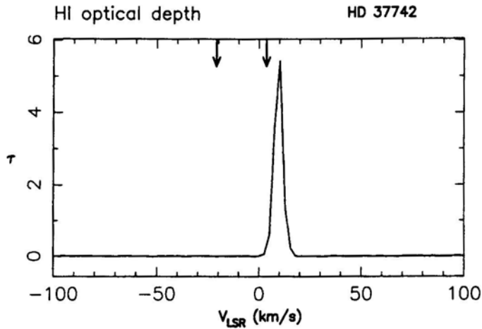
Figure 3. Spectram towards HD37742. The arrows on the velocity axis mark the velocities at which optical absorption is seen.
