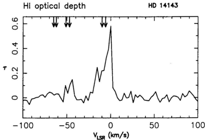
Figure 6. HI absorption spectra towards HD14143. The arrows mark the velocities at which optical absorption is seen.
