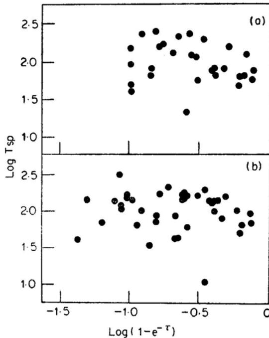
Figure 6a and b. The distribution of spin temperature versus optical depth for approximately 30 clouds measured in the Parkes survey (Radhakrishnan et al. 1972 b) a ; and for \sim 40 clouds measured recently by Mebold et al. (1980) b. For clouds with optical depths in this range, no definite trend is apparent in either distribution.
