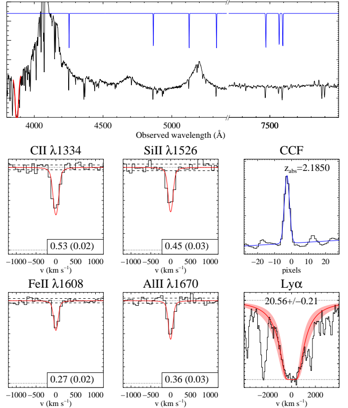
Fig. 3. Example of the SDSS spectrum of J152529.18+292813.18 with a DLA line at \lambda_{\text{obs}} \sim 3880 \text{ \AA} (top panel). The mask (template of low-ionisation absorption lines) used to derive an accurate redshift ( z_{\text{abs}} = 2.1850 ) from the cross-correlation function (shown in panel CCF with the origin of the pixel scale set from the first guess) is overplotted in blue in the upper panel. The automatic fits to a few metal absorption lines are shown in the left-hand side and middle panels (C II \lambda 1334 , Si II \lambda 1526 , Fe II \lambda 1608 , Al II \lambda 1670 ). Rest-frame equivalent widths and associated errors are indicated (in \text{\AA} ) at the bottom of each panel. The automatic Voigt-profile fit to the damped Ly- \alpha line is overplotted to the observed spectrum in the bottom-right panel. The shaded area corresponds to the uncertainty on the column density ( N(\text{H I}) = 10^{20.56 \pm 0.21} \text{ cm}^{-2} ).
