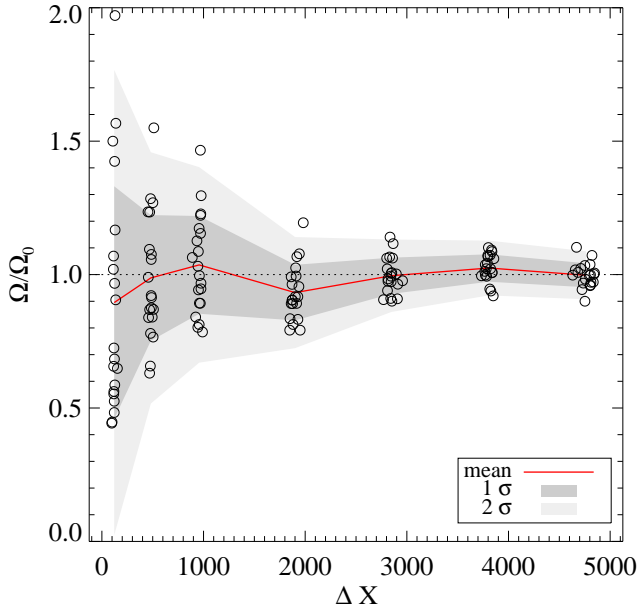
Fig. 16. Statistical uncertainty on the determination of \Omega_g^{\text{DLA}} as a function of the sample size. Each circle represents the ratio between the measurement of \Omega_g^{\text{DLA}} for a randomly selected sample of total absorption pathlength \Delta X ( \Omega ) and that obtained from the full SDSS sample, \Omega_0 . Note that \Delta X = 1\,540 , 8\,475 and 11\,099 in, respectively, Péroux et al. (2003), Prochaska & Wolfe (2009, after correcting for the edge-bias) and the present work.
