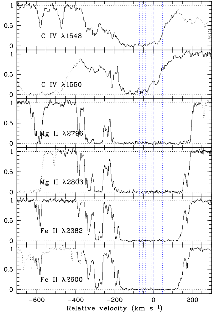
Fig. 2. Absorption profiles related to the C IV \lambda 1548, 1550, Mg II \lambda 2796, 2803 and Fe II \lambda 2382, 2600 transition lines. Blended parts of the profiles are shown by dotted histogrammes. The location of the C I-detected components (see Fig. 4) is indicated by vertical lines with the origin of the velocity scale corresponding to z_{\text{abs}} = 1.96221 .
