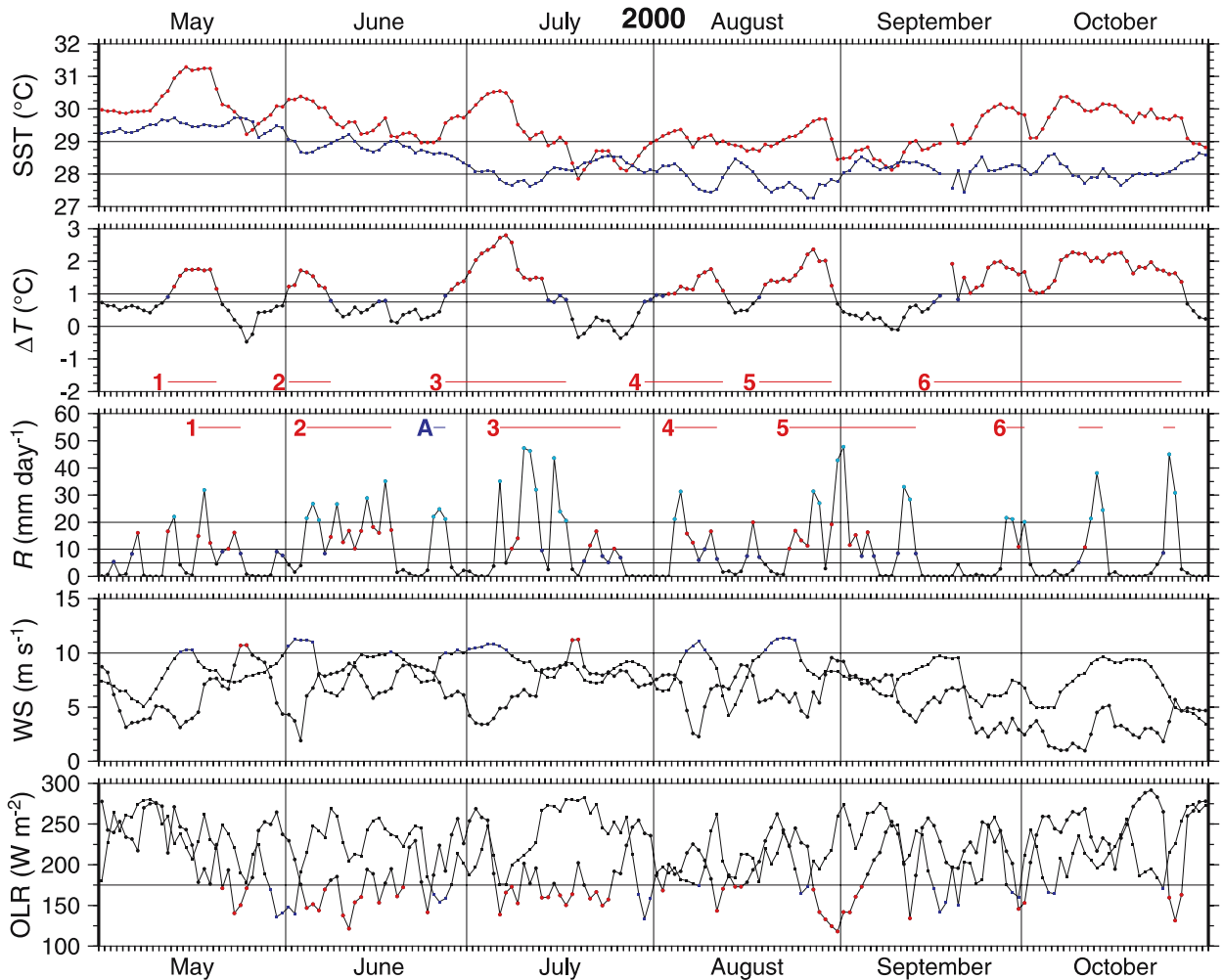
Figure 4. The first three panels are as in figure 2, but for 2000. See table 4 for a description of the events. The fourth (fifth) panel shows QuikSCAT wind speed ( \text{m s}^{-1} ) (OLR ( \text{W m}^{-2} )) in the northern (circles) and southern (squares) boxes. Wind speed \geq 10 \text{ m s}^{-1} is in red (blue) for the northern (southern) box. OLR \leq 175 \text{ W m}^{-2} is in red (blue) for the northern (southern) box. For a more detailed explanation of panels 4 and 5, see table 15 and section 4.7.
