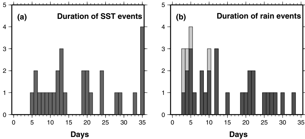
Figure 12. Histogram showing the frequency distribution of duration of SST and rain events. (a) SST events for the \Delta T \geq 0.75^\circ\text{C} criterion. Event 6 in 2000 was longer than 35 days, but has been clubbed with 35-day events. (b) Rain events that lag an SST event are shown as dark gray bars (total 28 events) and isolated rain events are shown as light gray bars (total 5 events). This histogram is for the \Delta T \geq 0.75^\circ\text{C} criterion. In the case of three events (Event 1 in 2001 and Events 2 and 3 in 2004), the duration shown excludes the multiple rain bursts associated with the SST event. Including the multiple bursts increases the duration to 58, 21, and 56 days from 12, 3, and 5 days for the three events. Note that the duration of SST events is less than that of associated rain events.
