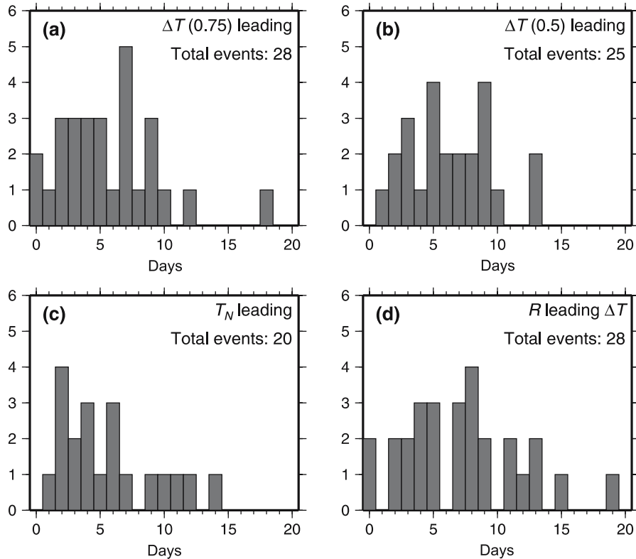
Figure 10. Lag histogram for the core monsoon period; the lag (in days) is on the abscissa. The figure shows the frequency distribution for different lags. (a) For SST events, defined on the basis of a \Delta T \geq 0.75^\circ\text{C} criterion, leading a rainfall event during the core monsoon period (Experiment C in table 12); see table 11 for a summary of these events. (b) For SST events, defined on the basis of a \Delta T \geq 0.5^\circ\text{C} criterion (Experiment 2 in table 12). (c) For SST events, defined on the basis of a T_N \geq 29^\circ\text{C} criterion (Experiment 5 in table 12), leading a rainfall event during the core monsoon period. The number of events depends on the criterion used to define them. (d) Histogram (during the core monsoon period) for the lag between the ending of a rain event and the start of the succeeding SST event based on the \Delta T \geq 0.75^\circ\text{C} criterion. This histogram is complementary to that in (a).
