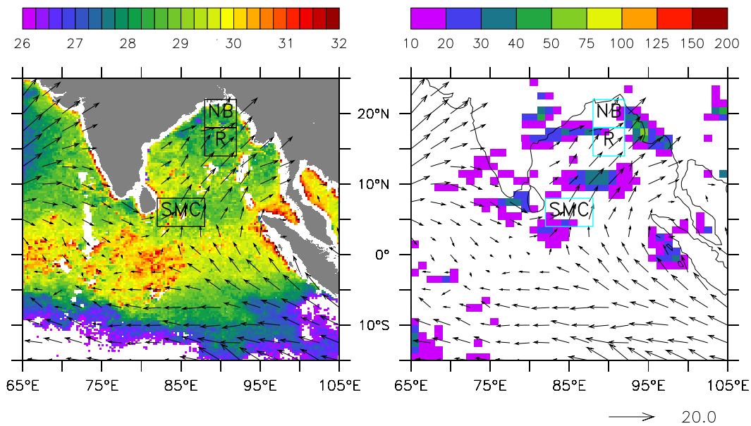
Figure 1. The panel on the left shows TMI SST (colour, ^{\circ}\text{C} ) and the panel on the right shows GPCP rainfall (colour, \text{mm day}^{-1} ). Superimposed on both panels are QuikSCAT wind vectors ( \text{m s}^{-1} ); the vector scale is at the bottom right corner of the right panel. The data are plotted here for 1 August 2003. Boxes are shown defining the regions over which SST and rainfall are averaged. In the northern bay, SST is averaged over 82^{\circ} – 88^{\circ}\text{E} and 18^{\circ} – 22^{\circ}\text{N} ; in the southern bay, SST is averaged over 82^{\circ} – 88^{\circ}\text{E} and 4^{\circ} – 8^{\circ}\text{N} , the regime of the SMC. Rainfall is averaged in the central bay over 88^{\circ} – 92^{\circ}\text{E} and 14^{\circ} – 18^{\circ}\text{N} .
