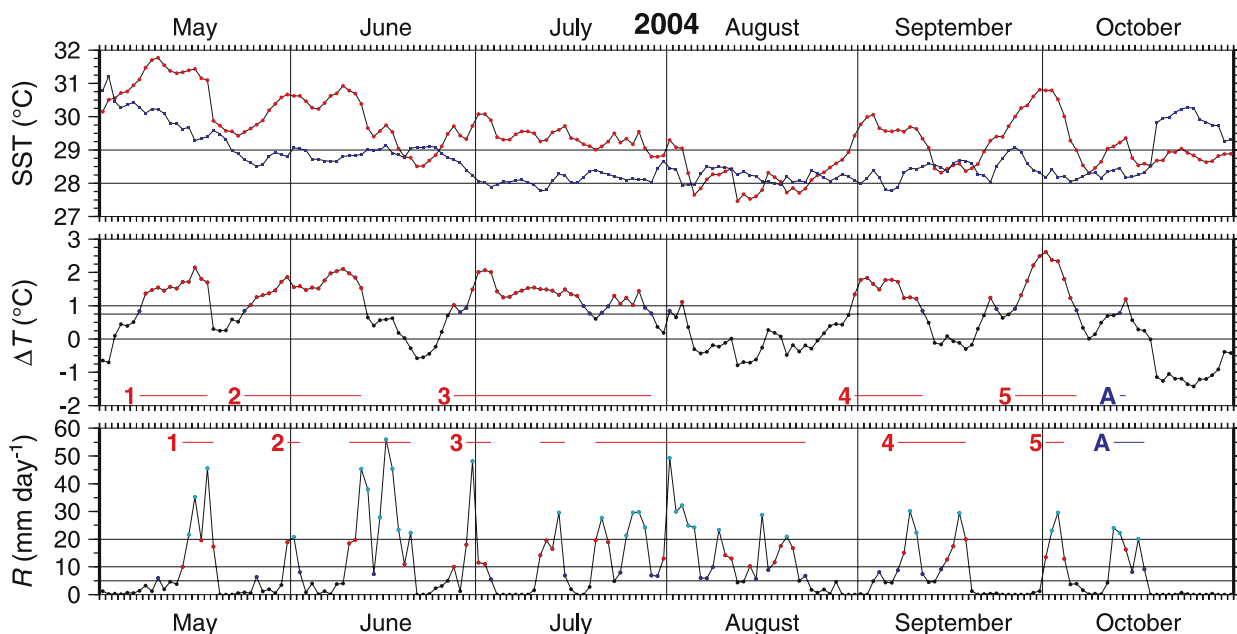
Figure 8. As in figure 2, but for 2004. See table 8 for a description of the events.
