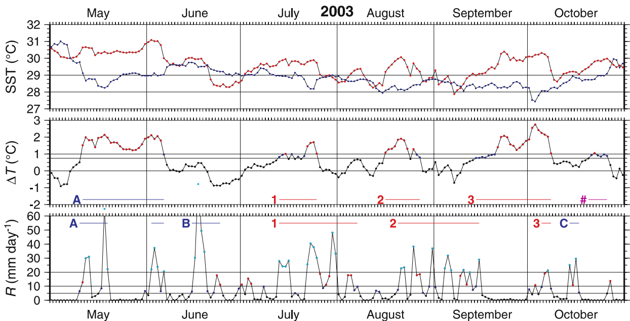
Figure 7. As in figure 2, but for 2003. See table 7 for a description of the events.
