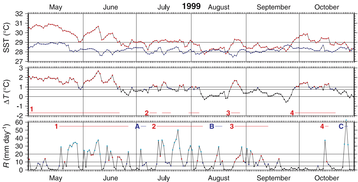
Figure 3. As in figure 2, but for 1999. See table 3 for a description of the events.
