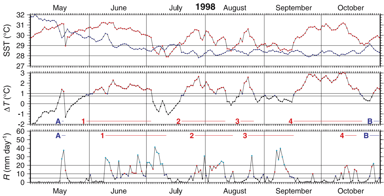
Figure 2. SST, SST difference, and rainfall for 1998. The first panel shows TMI SST ( ^{\circ}\text{C} ) in the northern (red circles) and southern (blue squares) boxes. The second panel shows the SST difference ( \Delta T ) between the northern and southern boxes; black symbols are used for \Delta T < 0.75^{\circ}\text{C} , blue for 0.75^{\circ}\text{C} \leq \Delta T < 1^{\circ}\text{C} , and red for \Delta T \geq 1^{\circ}\text{C} . The third panel shows rainfall ( R , \text{mm day}^{-1} ); black symbols are used for R < 5 , blue for 5 \leq R < 10 , red for 10 \leq R < 20 , and light blue for R \geq 20 . In panels 2 ( \Delta T ) and 3 (rainfall), the duration of an event is shown by a line. Events in which SST leads rainfall are in red, and isolated rainfall (SST) events are in blue (magenta). The event number precedes the line showing its duration. Line segments without a preceding event number indicate continuation of the previous event (see condition 5 in the definition of SST and rainfall events). See table 2 for a description of the events.
