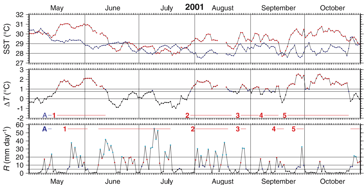
Figure 5. As in figure 2, but for 2001. See table 5 for a description of the events.
