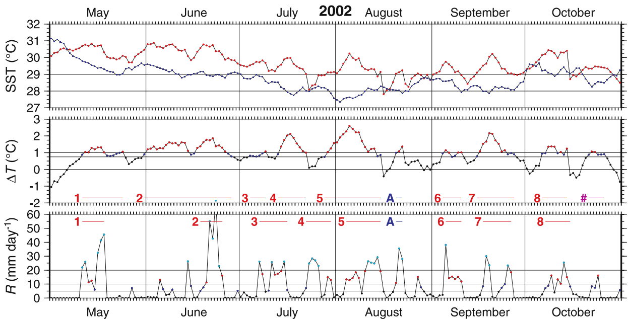
Figure 6. As in figure 2, but for 2002. See table 6 for a description of the events.
