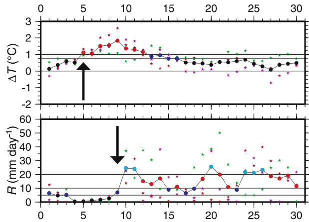
Figure 11. \Delta T (top panel) and rainfall for a composite of events with four-day lag (SST leading rainfall). The three events with a four-day lag are Event 3 in 1998 (figure 2 and table 2), Event 2 in 1999 (figure 3 and table 3), and Event 2 in 2003 (figure 7 and table 7). The abscissa is in days, with Day 5 marking the start of the individual and composite SST events. The arrows mark the start of the composite (and individual) SST and rain events. The composite of the events is shown by the solid line and filled circles in both panels. Black circles are used for \Delta T < 0.75^\circ\text{C} , blue for 0.75^\circ\text{C} \leq \Delta T < 1^\circ\text{C} , and red for \Delta T \geq 1^\circ\text{C} . Black circles are used for R < 5 , blue for 5 \leq R < 10 , red for 10 \leq R < 20 , and light blue for R \geq 20 . The individual events are shown by coloured asterisks (dark red for 1998, green for 1999, and magenta for 2003).
