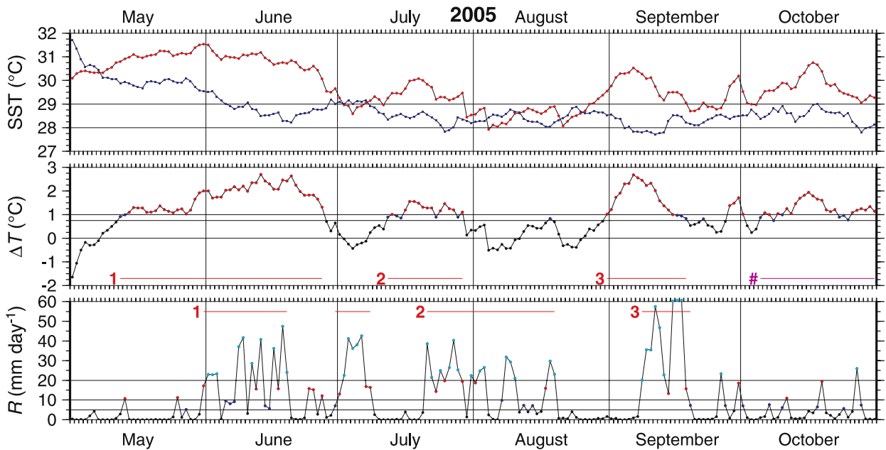
Figure 9. As in figure 2, but for 2005. See table 9 for a description of the events.
