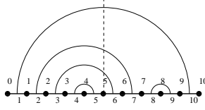
FIGURE 1. The element S \in Hom([10], [0])
