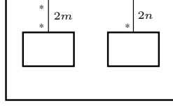
FIGURE 8. Multiplication in Gr_0(P)
