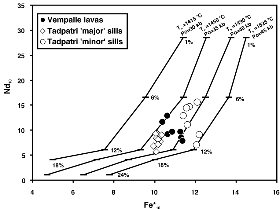
Fig. 13. Variation in \text{Fe}_{10}^* and \text{Nd}_{10} during polybaric accumulated fractional melting of a fertile peridotite KLB-1 (after Langmuir et al. , 1992). These are assumed to represent point and depth average compositions of melts in a 'column' of mantle undergoing adiabatic decompression. Bulk-rock \text{FeO}^* and Nd contents are normalized to 10 wt % MgO for samples with LOI < 3 wt %.
