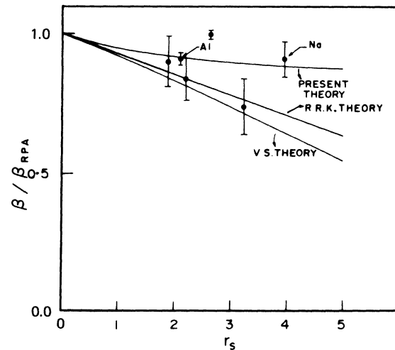
FIG. 2. Plasma dispersion parameter \beta/\beta_{RPA} in various theories (see text). Experimental results (Ref. 9) for Be, Al, Sb, Mg, Li, and Na in order of increasing r_s are also shown.
