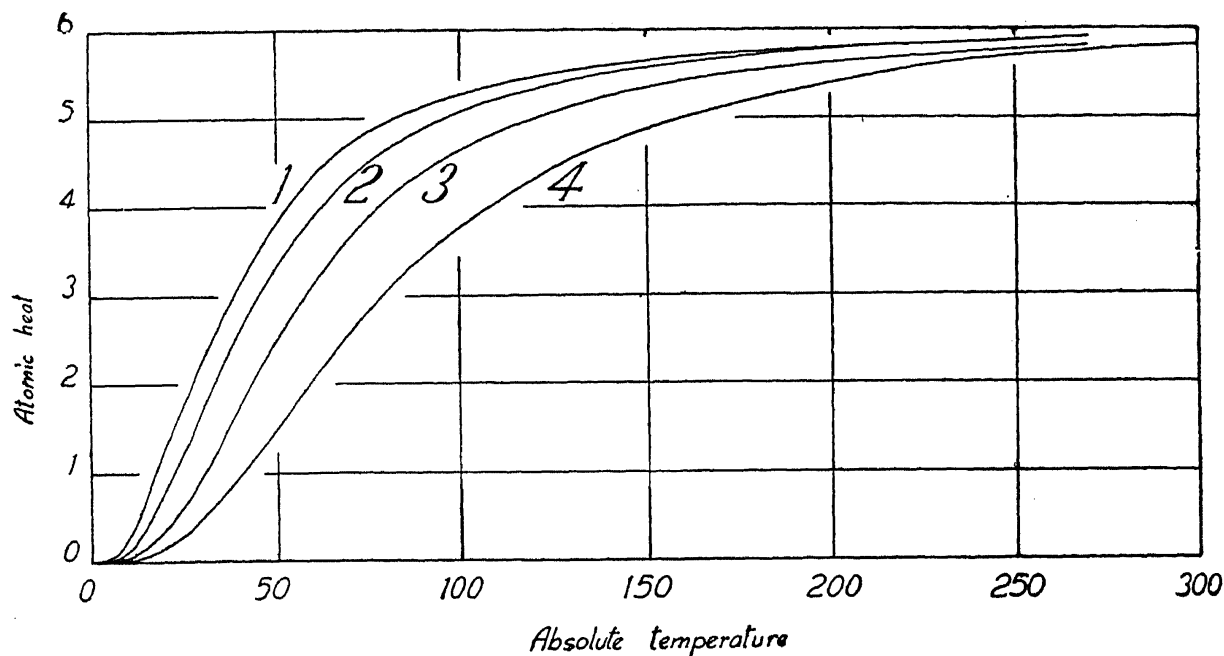
FIG. 1. Experimental Values of the Atomic Heats. (1) KI, (2) KBr, (3) KCl and (4) KF.
