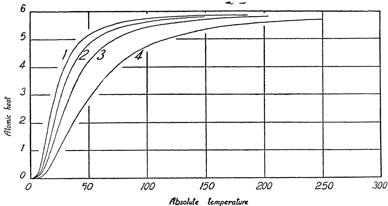
FIG. 2. Computed Values of the Atomic Heats. (1) RbI, (2) RbBr, (3) RbCl and (4) RbF.
