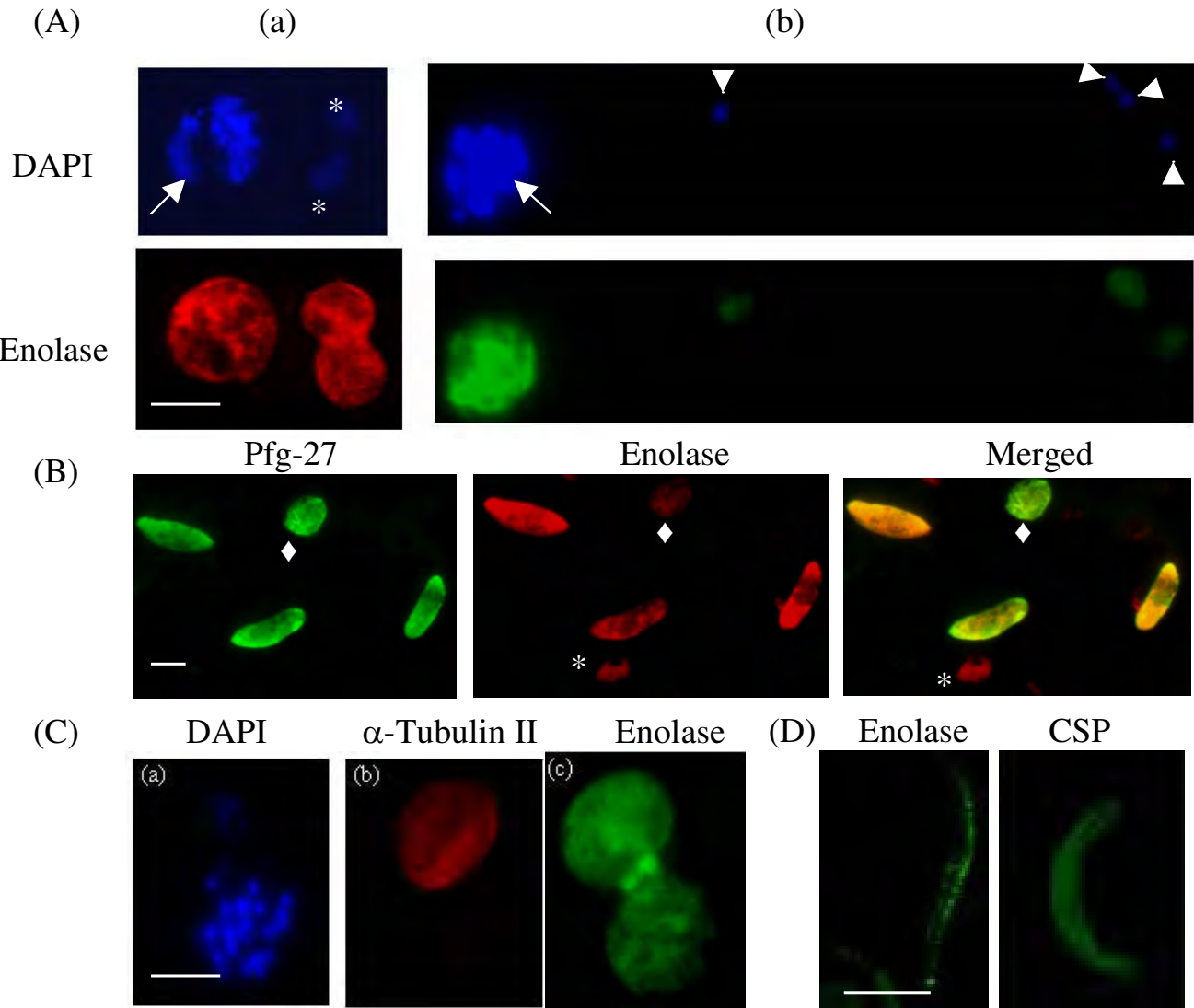
Figure 1 Immunofluorescence assays (IFA) for the localization of enolase at different stages of Plasmodium life cycle. (A) Asexual stages, (B) Gametocytes, (C) Gamete (mosquito stage) and (D) Sporozoite (mosquito salivary gland stage). Sporozoite preparation was from P. yoelii , while all other stages shown are for P. falciparum . Ring stages (triangle), trophozoite (*), schizont (→) and stage II gametocyte (diamond). Different fluorescent probes used were, (i) DAPI as a nuclear marker, (ii) mouse anti-r-Pfen (green), (iii) rabbit anti-r-Pfen (red), (iv) mouse anti-Pfg-27 (green) as gametocyte marker, (v) rabbit anti-male gametocyte specific \alpha -tubulin II antibody (red) and (vi) mouse anti-CSP antibody (green) as sporozoite surface marker. The scale bars shown corresponds to 5 \mu m.
