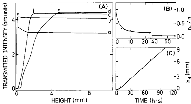
FIG. 1. (a) Transmitted intensity as a function of height in the suspension cell containing 0.109- \mu\text{m} -diam particles at n = 4.2 \times 10^{12} \text{ cm}^{-3} at different times after the addition of the ion-exchange resins: a , 0.1 h; b , 4.2 h; c , 22 h; d , 54 h. Vertical arrows indicate the position of the interface between the dense and the rare phases. (b) Concentration in the rare phase relative to n as a function of time. (c) Height of the dense phase ( h_d ) as a function of time.
