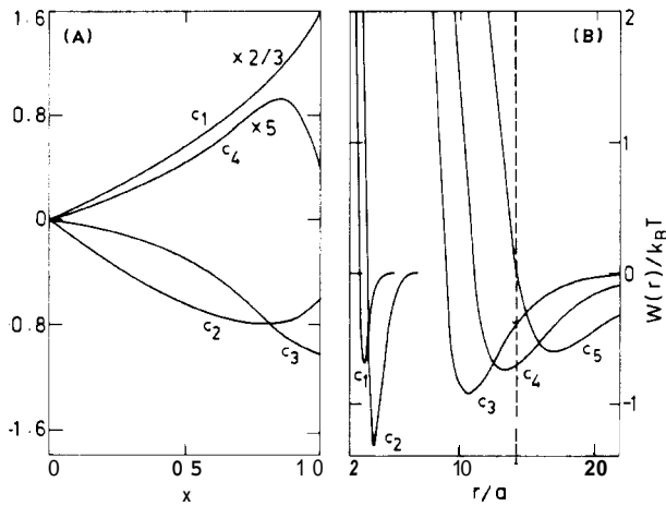
FIG. 2. (a) The difference in the free energy \Delta F(x) relative to the thermal energy Nk_B T as a function of the fraction x for various impurity concentrations C expressed relative to the counterion concentration nZ ( c = C/nZ ): c_1 = 170 , c_2 = 60 , c_3 = 3 , and c_4 = 1.5 . The value of \phi is 0.284%. (b) The effective interparticle potential W(r) relative to k_B T for various values of c . c_1 to c_4 : same as those in (a); c_5 = 0.5 . Vertical dashed line shows the position of average interparticle separation R for \phi = 0.284\% .
