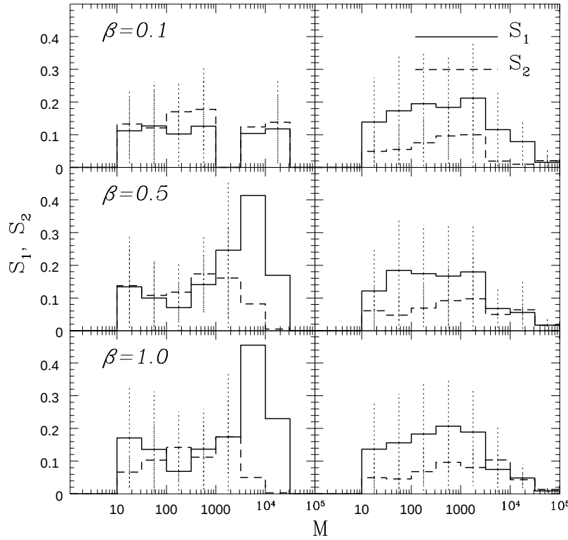
Figure 2. The shape of clusters at the percolation threshold is shown for the IRAS 1.2 Jy catalogue (left) and the randomized IRAS catalogue (right). S_1 represents filamentarity and S_2 planarity. For more details see Sathyaprakash et al [14].
