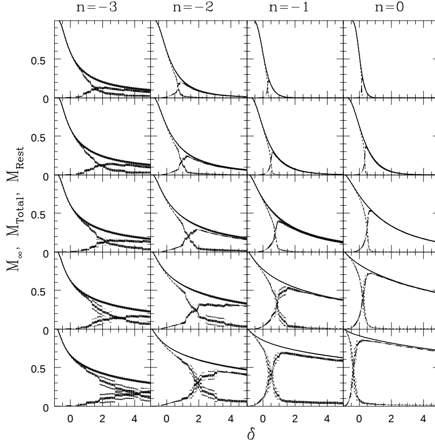
Figure 1. Percolation curves are shown for an N -body simulation evolving under gravitational instability from Gaussian initial conditions with a scale free initial spectrum P(k) = k^n , n = -3, -2, -1, 0 . The cosmological epoch increases from top to bottom and the primordial spectrum increases from left to right. The dotted line corresponds to M_\infty , the mass fraction in the largest cluster; M_{\text{Rest}} corresponds to the mass fraction in all clusters with the exception of the largest; M_{\text{Total}} is the mass fraction in all clusters above a given density threshold, M_{\text{Total}} = M_\infty + M_{\text{Rest}} . The percolation transition is characterised by a sharp increase in M_\infty . The value of M_{\text{Rest}} is sharply peaked just before the onset of percolation indicating that the number of clusters is maximum at this threshold. For more details see Sathyaprakash, Sahni and Shandarin [12].
