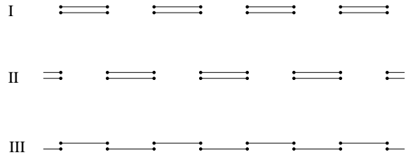
FIG. 1: The three degenerate ground states. Each solid circle represents a spin 1/2, and the lines denote singlet bonds.
