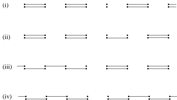
FIG. 2: Various possible excitations interpolating between different ground states. The lines denote singlet bonds, and each isolated circle denotes a free spin 1/2 .
