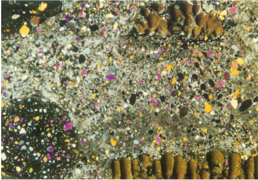
Figure 6. Thin section of eggs (brown colour) in pedogenically modified calcareous sandstones. Rounded caliche nodule to the left is 1 cm in diameter.
