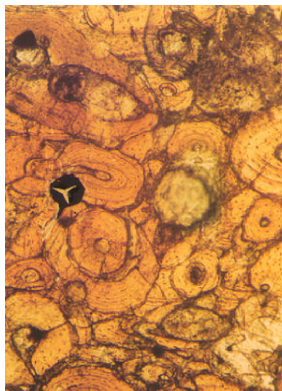
Figure 5. Cross-section of sauropod bone from Anjar showing growth and well-preserved osteons marked by arrows. Osteon diameters are about 25 \mu\text{m} .
