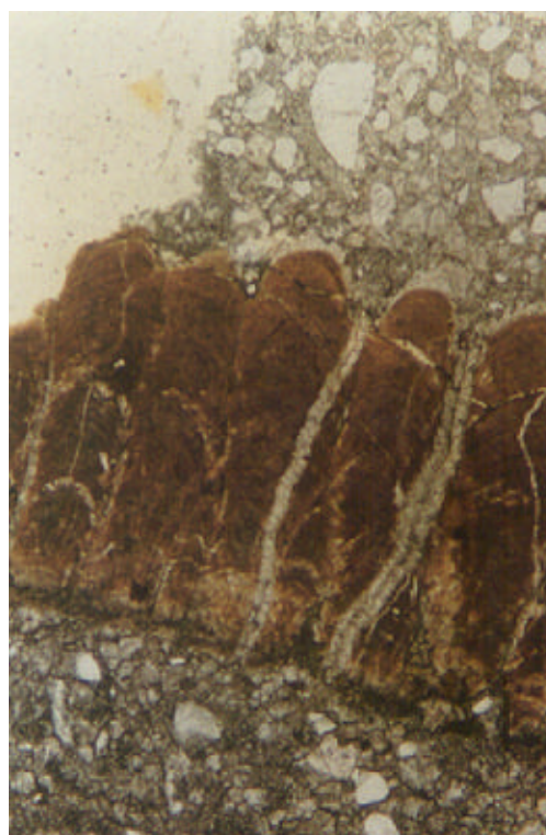
Figure 9. Thin section of sauropod eggshell showing calcitic spherulites and air canals running through the shell. Shell thickness about 2.5 mm.
