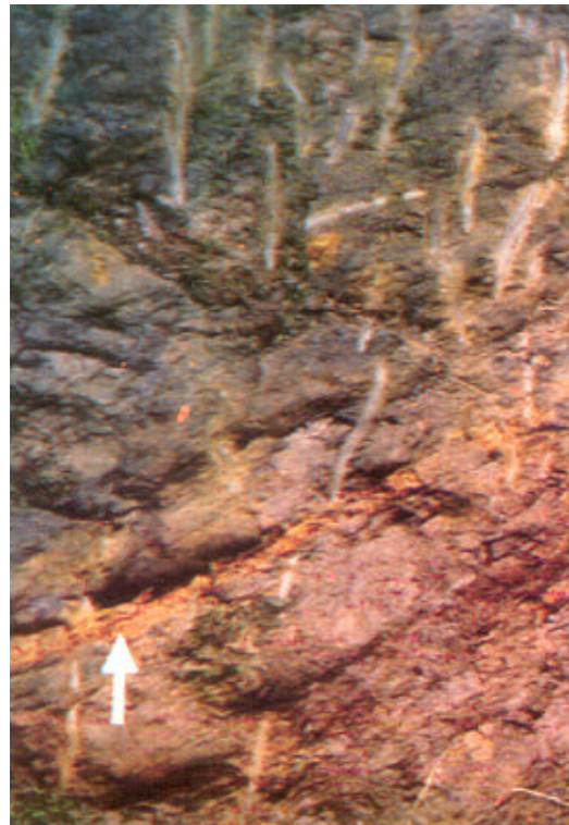
Figure 12. Section at Um Shorengkew in Meghalaya showing iridium-enriched layer marking (with arrow) the fallout of the asteroid impact. (Photo: Courtesy Bhandari et al. 23 ).
