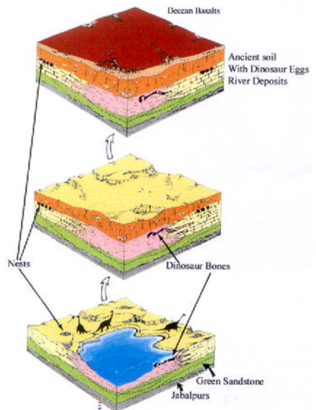
Figure 7. Stages in the preservation of eggs, nests and bones at Jabalpur.
