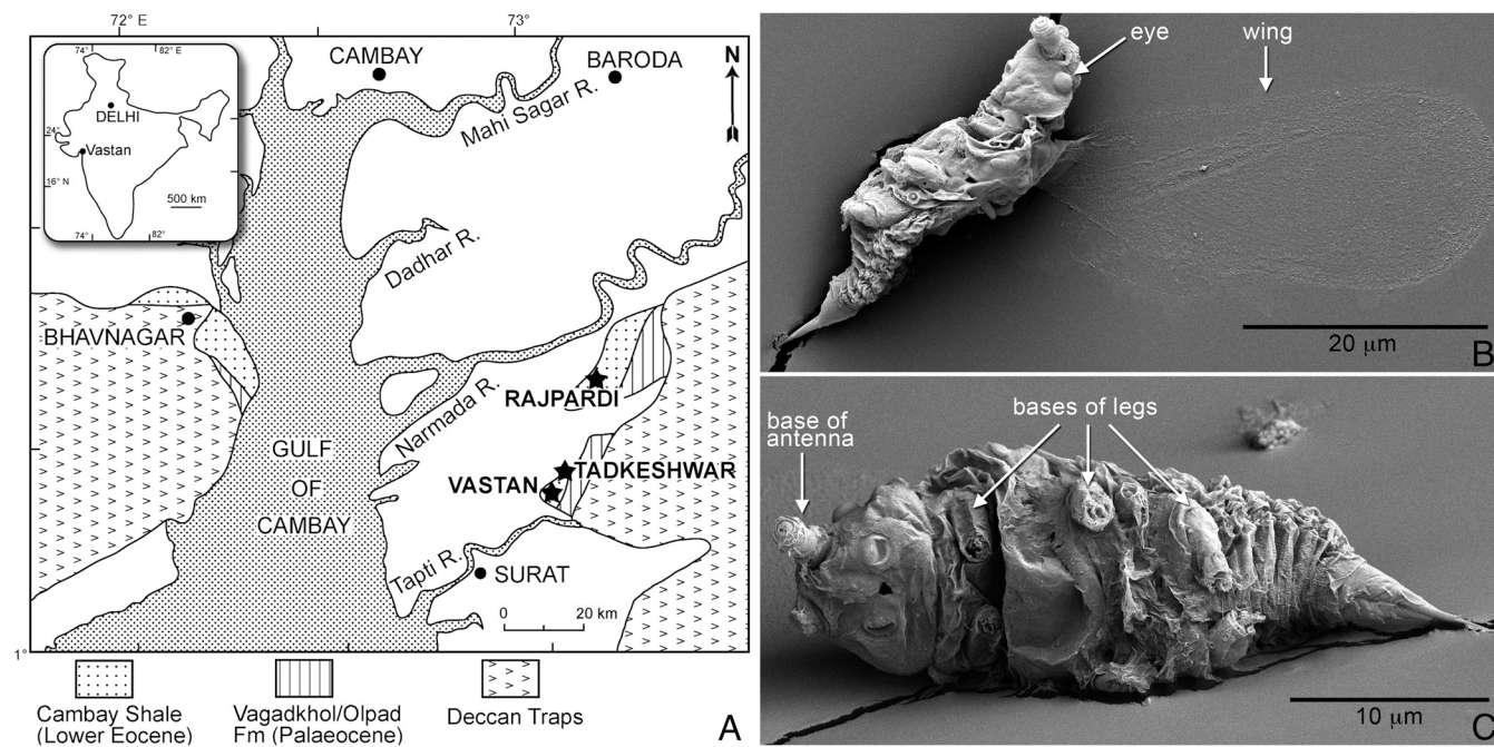
Fig. 1. (A) Map showing location of mines and distribution of formations yielding Early Eocene Cambay amber from Gujarat, India. (B and C) Scanning electron micrographs of male scale insect (Neococcoidea), fully extracted from Cambay amber using solvents; (B) oblique dorsal view with wing outstretched, (C) ventral view.
