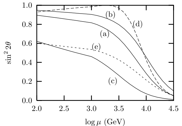
Figure 1: \sin^2 2\theta has been plotted against the renormalization scale. The values of M_H , \mu_0 and M are 115 GeV, 1 TeV and 30 TeV, respectively. The different plots correspond to different combinations of (d\kappa|_M, \sin^2 2\theta|_M) given by: (a) (1.5 \times 10^{-4}, 0.05) , (b) (1.5 \times 10^{-4}, 0.1) , (c) (1.5 \times 10^{-4}, 0.01) , (d) (1.3 \times 10^{-4}, 0.05) , and (e) (1.7 \times 10^{-4}, 0.05) .
