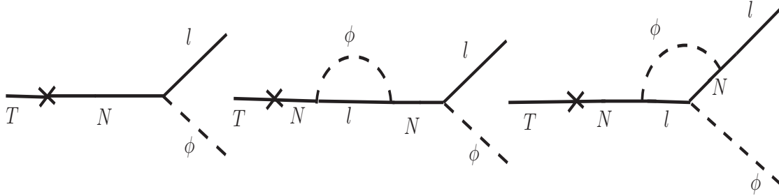
Figure 2: The tree and one-loop level contribution to the decay of T_1 that generate the lepton asymmetry.
