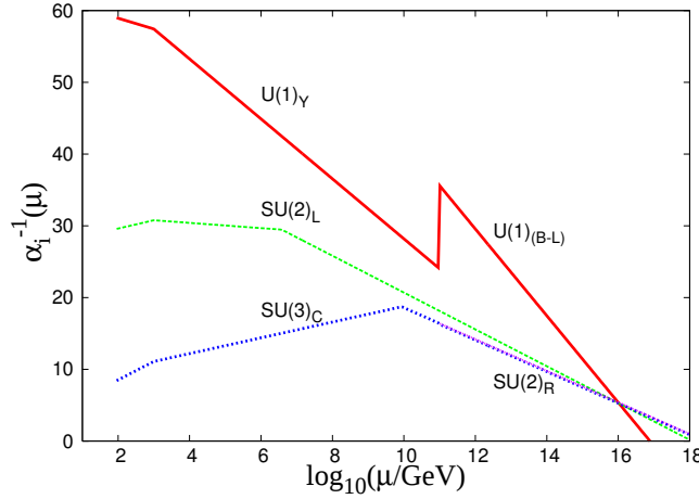
Figure 1: Unification of gauge couplings with left-right symmetry breaking at M_R = 10^{11} GeV with n_\sigma = n_C = 3 (see text). Below M_U = M_P = 10^{16} GeV, g_L \neq g_R . The SU(3)_C coupling (short-dashed line) and the SU(2)_R coupling (dotted line) appear to merge for \mu > M_R because fortuitously, in this example, the beta-function coefficients for both are nearly equal in this energy range as are the boundary values of the two couplings at M_R .
