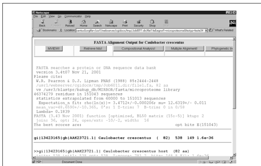
Figure 3. Parsed FASTA report of query Hfq RNA binding protein for hits against C. crescentus obtained after clicking the "FASTA Output" in the proteome-wise FASTA report from Figure 2. The report is similar in structure to that obtained from typical FASTA searches against standard protein databases. The screenshot shows the various options available for the post-processing of FASTA output.
