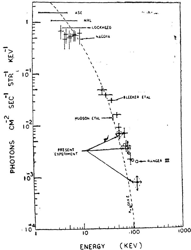
FIG. 3. The omnidirectional X-ray flux at the top of the atmosphere.
