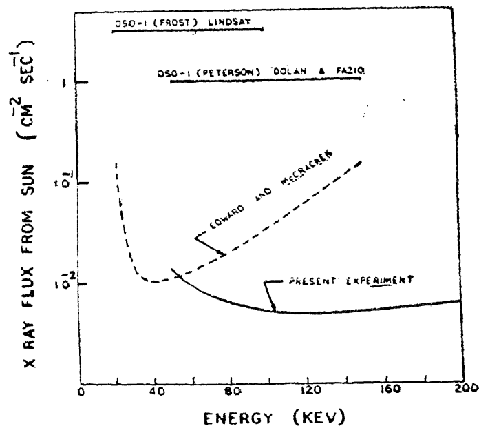
FIG. 4. The upper limit for the emission of hard X-rays from the sun.
