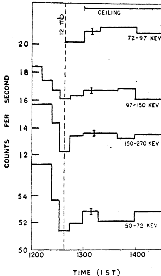
FIG. 2. The counting rates of X-rays of different energies as a function of time near the ceiling altitude.
