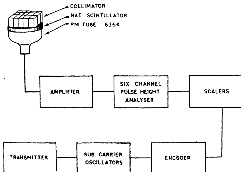
FIG. 1. The block diagram of the balloon-borne X-ray detector.
