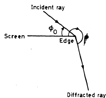
Figure 1. Diffraction geometry: parallel rays incident on a straight edge at a glancing angle of \phi_0 .
