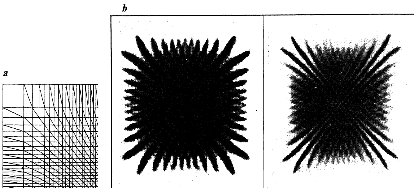
Figure 5. a , Positions of intensity maxima for a 90° sector as obtained from geometrical theory of diffraction. b , Diffraction pattern for a square disc: monochromatic light (left) and white light (right). (After Kathavate 17 )
