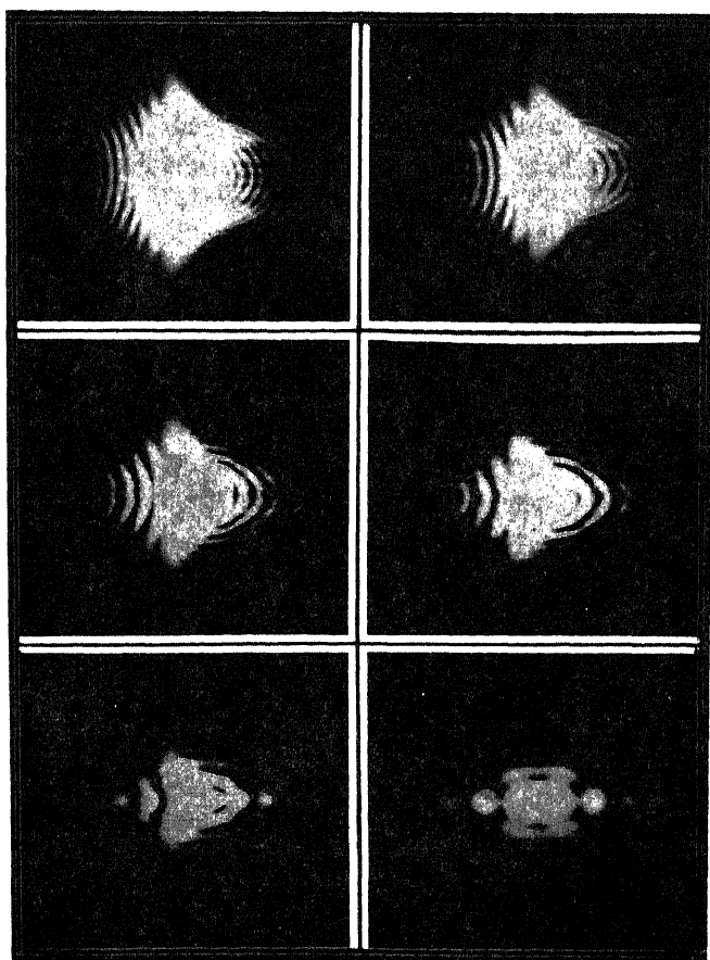
Figure 4. Transition from Fresnel to Fraunhofer diffraction pattern in the case of a semicircular aperture. (After Kathavate 17 )
