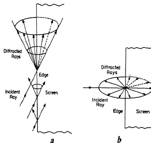
Figure 2. Diffracted rays can be obtained from the Rubinowicz 'reflection' condition. a , Diffracted rays will be on a cone symmetric about the edge for an oblique incidence. b , Diffracted rays will be on a disc perpendicular to the edge for normal incidence.
