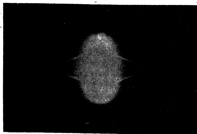
Figure 3. Diffraction caustic of an elliptical aperture. (After Raman 16 )
