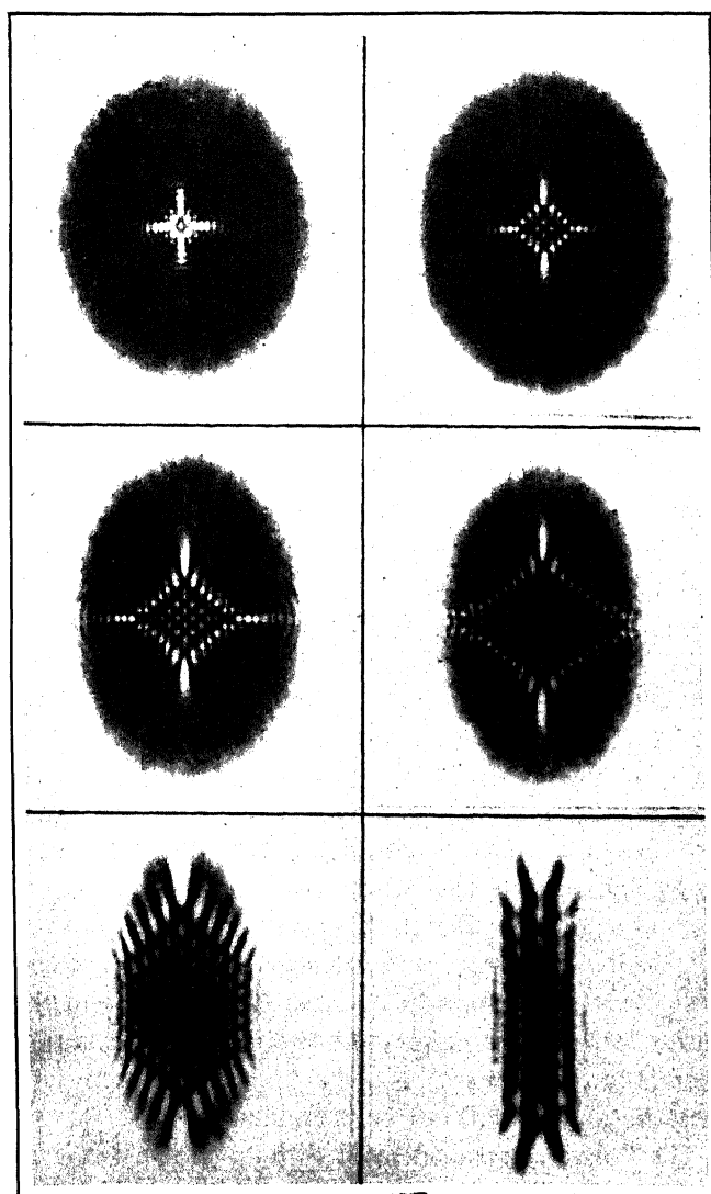
Figure 6. Diffraction pattern within the shadow of an elliptic disc. The picture shows the effect of increasing eccentricity. (After Kathavate 17 )
