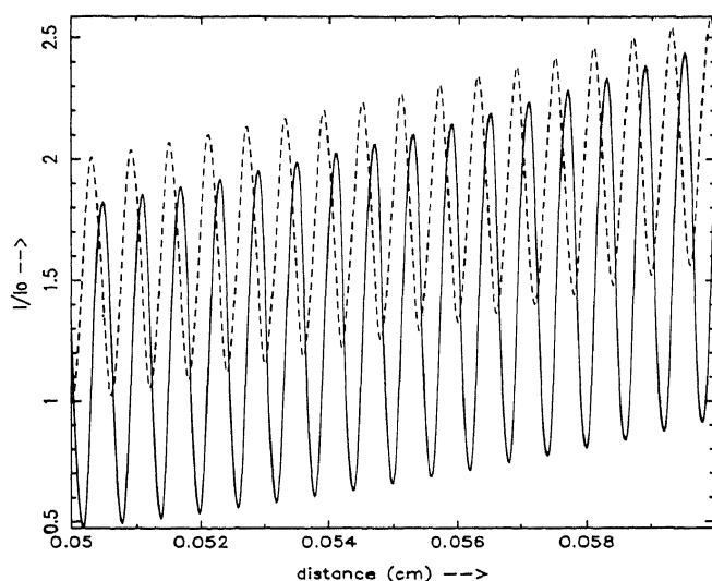
Figure 7. Calculated intensity pattern in the shadow region of a strip (full line) and a cylinder of equal width (dashed line).
