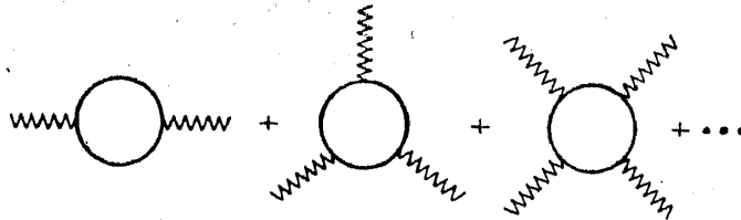
Figure 1. Closed loop diagrams corresponding to the series in eq. (14). Wavy lines and ordinary lines denote the gluons and quarks respectively.
