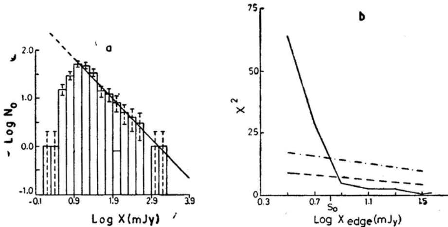
Figure 3. Same as in Fig. 2, with X = S/\{\beta(1 + T_{\text{sky}}/T_r) (1 + K_2D/P)^{1/2} (\cos \delta)^{1/2}\} .
