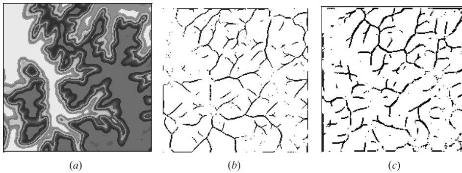
Figure 5. (a) DEM after Gaussian blurring with a 3-pixel radius; (b) VCN; and (c) RCN.
