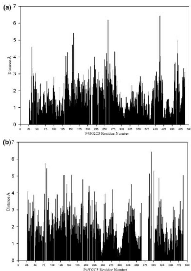
Fig. 9 Distance variation in C \alpha backbone position in (a) P-450 2C5 (1 N6B) versus P-450 1A1 liver model and (b) P-450 2C5 (1 N6B) versus P-450 1A1 brain variant model. PROFIT was used to give a by-residue distance difference analysis from the least squares fit of the two models compared to the template P-450 2C5 coordinates used to generate the models. The zones used for initializing the superimposition were supplied from the alignment in Fig. 8 and fitted based on C \alpha carbons. The overall C \alpha carbon RMSDs were 2.051 Å and 2.354 Å for liver and brain variant P-450 1A1, respectively. The abscissa represents the P-450 2C5 residue number. The P-450 2C5 residue numbers without a corresponding C \alpha carbon in liver or brain variant P-450 1A1 are seen as breaks in the data, which essentially depicts gaps in the structural alignment.
