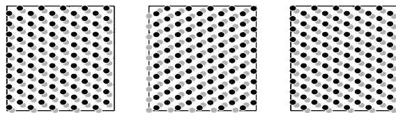
FIG. 2: Simulation images of macroscopically ordered lattices drifting through each other for \epsilon = 0.05 , F_d^* = 0.0438 .
