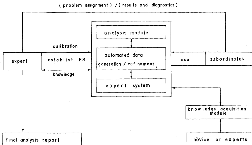
Figure 2. Role of expert systems in finite element analysis.
