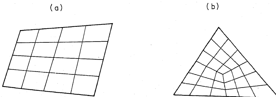
Figure 8. Initial mesh patterns: (a) quadrilateral surface, (b) triangular surface.
