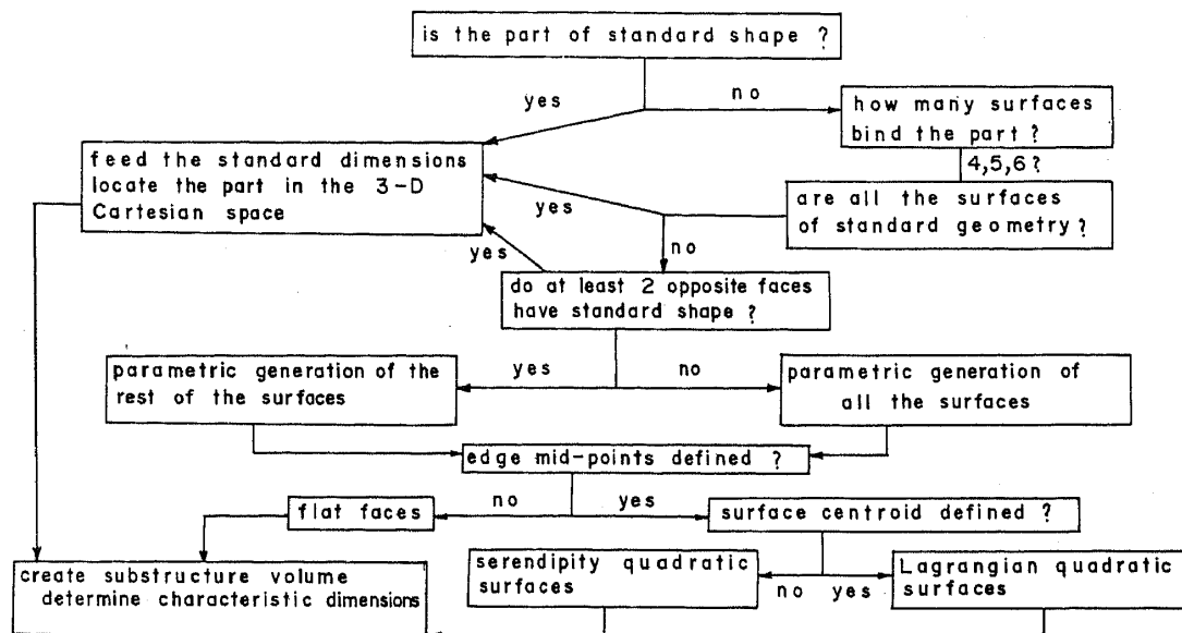
Figure 5. Flow of logic for geometric data generation.
