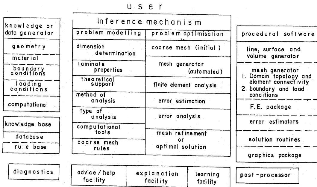
Figure 4. Blackboard architecture for expert system in adaptive finite element analysis.
