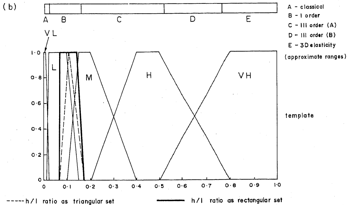
Figure 7. Fuzzy sets for the dimension ratios: (a) generation of dimension ratios; (b) comparison of fuzzy sets.
