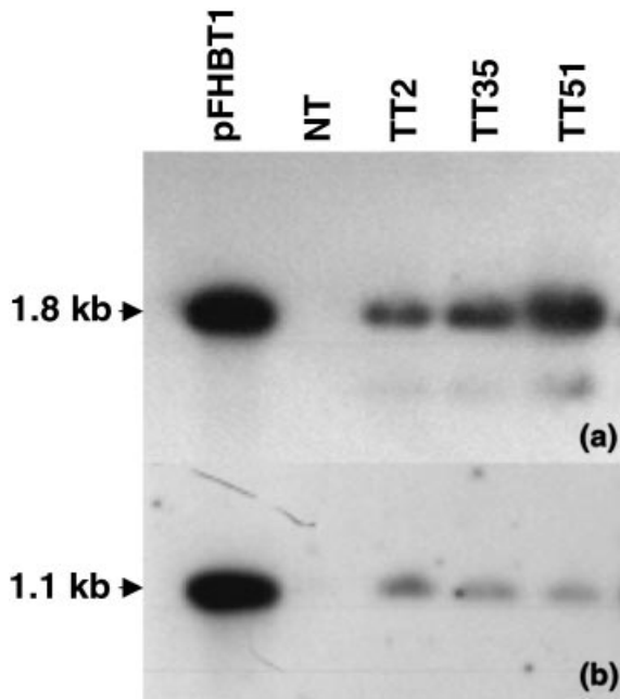
Figure 2 Southern blot analysis of T_0 transgenic plants. A total of 5 \mu g of plant genomic DNA and 30 \mu g of plasmid DNA were digested with the indicated coding sequence cutters for each gene and electrophoresed on 1% (w/v) agarose gels. The blots were then hybridized with (a) a Bt -specific probe and (b) an hph -specific probe. The arrows mark the expected 1.8 kb fragment-digested Bt plasmid DNA of pFHBT1 and 1.1 kb digested hph plasmid DNA of pGL2RC7. NT: non-transformed Minghui 63 control plant; TT2, TT35 and TT51: three T_0 transgenic plants.
