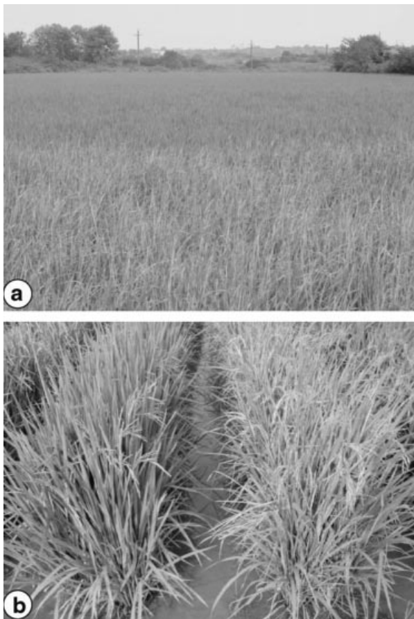
Figure 10 Field reactions of transgenic restorer line against stem borers. (a) Resistance reaction of restorer line against leaf-folders: Minghui 63/ Bt plants (top) and Minghui 63 control plants (bottom); (b) Resistance reaction of restorer line against yellow stem borers: Minghui 63/ Bt plants (left) and Minghui 63 control plants (right).
