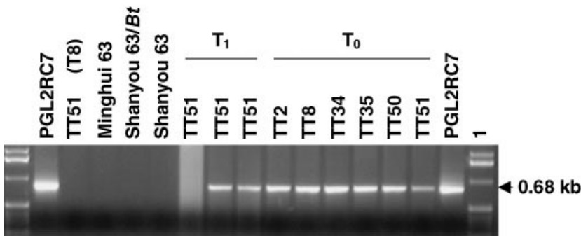
Figure 9 PCR analysis of hph transgenes in different generations. TT51-1 (T8): the eighth generation of the transgenic line TT51-1; Minghui 63: the non-transgenic control; Shanyou 63/ Bt : the Bt hybrid derived from the cross of TT51-1 with CMS line Zhenshan 97; Shanyou 63: the non-transgenic hybrid control; TT51-1, 4, 5: three T1 plants of TT51; TT2, TT8, TT34, TT35, TT50, TT51: the primary transgenic plants; pGL2RC7: the plasmid that contains the hph and chitinase genes and that was used for the co-transformation with Bt plasmid in the experiment.
