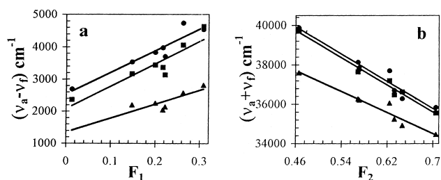
Fig. 2. (a) Plot of (\nu_a - \nu_f) against the polarity parameter F_1 = \{(\epsilon - 1)/(2\epsilon + 1) - (n^2 - 1)/(2n^2 + 1)\} (see Eq. (2)) for (●) STQ-1, (■) STQ-2 and (▲) STQ-3. (b) Plot of (\nu_a + \nu_f) against the polarity parameter F_2 = \{(\epsilon - 1)/(2\epsilon + 1) + (n^2 - 1)/(2n^2 + 1)\} (see Eq. (3)) for (●) STQ-1, (■) STQ-2 and (▲) STQ-3.
