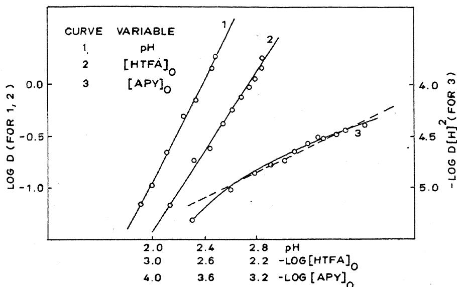
Figure 2. \text{UO}_2 -HTFA-APY- \text{CCl}_4 : log-log plots.
