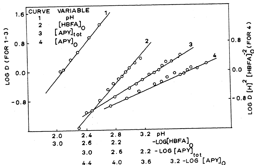
Figure 1. \text{UO}_2\text{-HBFA-APY-CCl}_4 : log-log plots.
