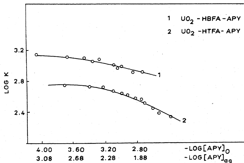
Figure 3. Variation of \log K with [\text{APY}] .
