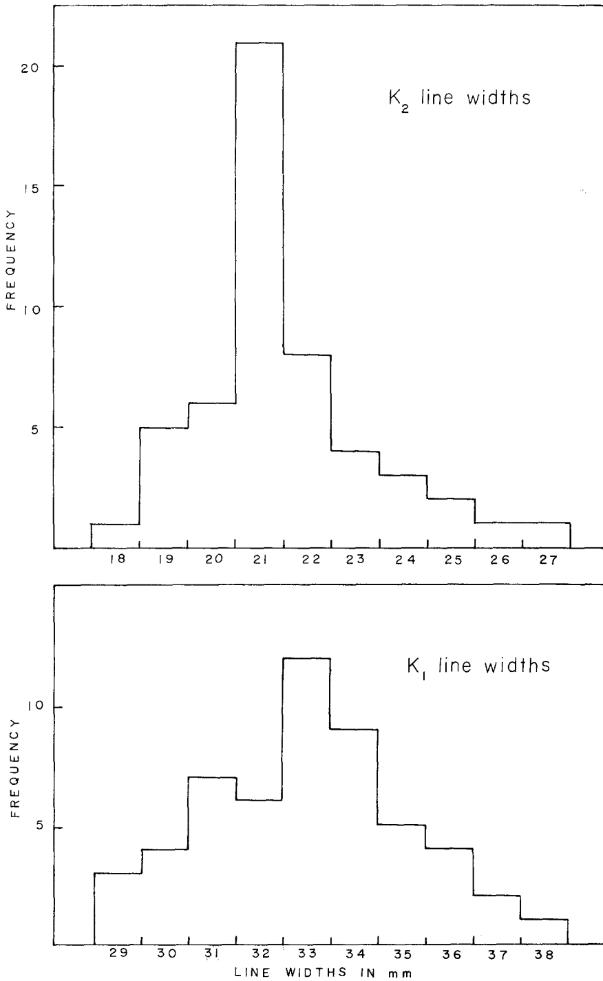
Fig. 7. Distribution of K 2 and K 1 -line widths measured from 52 profiles having measurable K 2V and K 2R . Abscissa gives line widths measured in mm on the tracings (1 mm = 1,268 km/sec).
