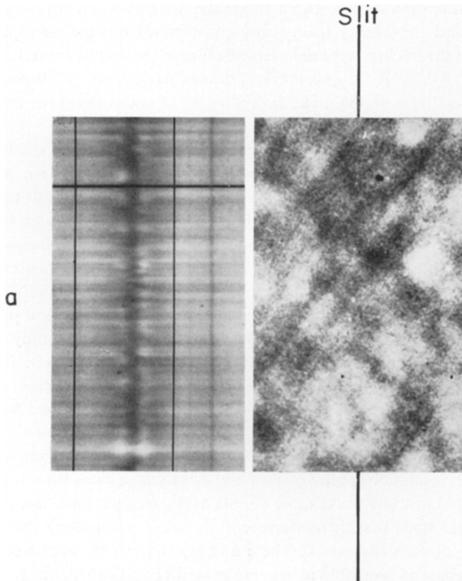
Fig. 1a. The K-line spectrogram of 12 June 1964, Scale:5.5"/mm. The 2 vertical dark lines are shadows of wires stretched in the focal plane. The horizontal dark line is caused by a wire stretched across the entrance slit of the spectrograph.
