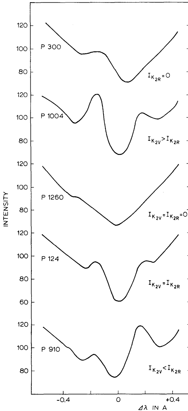
Fig. 2. Samples of profiles at 5 points along the slit showing different ratios of I_{K_{2V}} and I_{K_{2R}} . The numbers P 300 etc. give the profile designation along the slit, reckoned from the wire shadow parallel to the dispersion.
