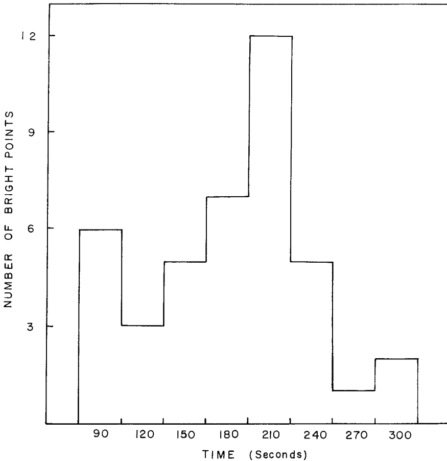
Fig. 9. Distribution of life times of bright points.
