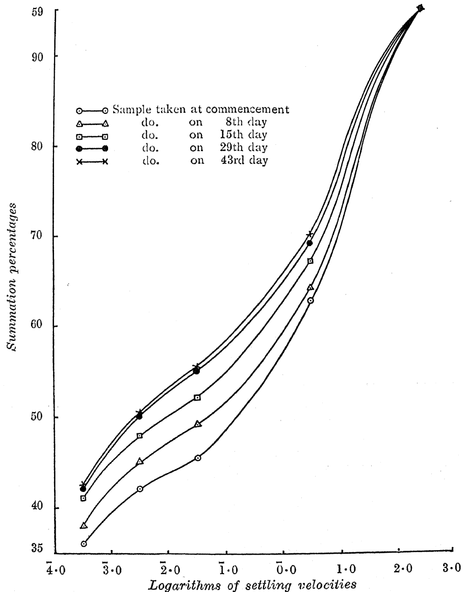
FIG. I. Size distribution of mineral matter.
