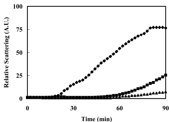
Fig. 4. Photo-induced aggregation of 0.2 mg/ml of \gamma -crystallin in the absence (◆) and in the presence (■) of 0.2 mg/ml and (▲) 0.4 mg/ml of 70S ribosome at 37°C. Aggregation was measured by monitoring the scattering of 475 nm light.
