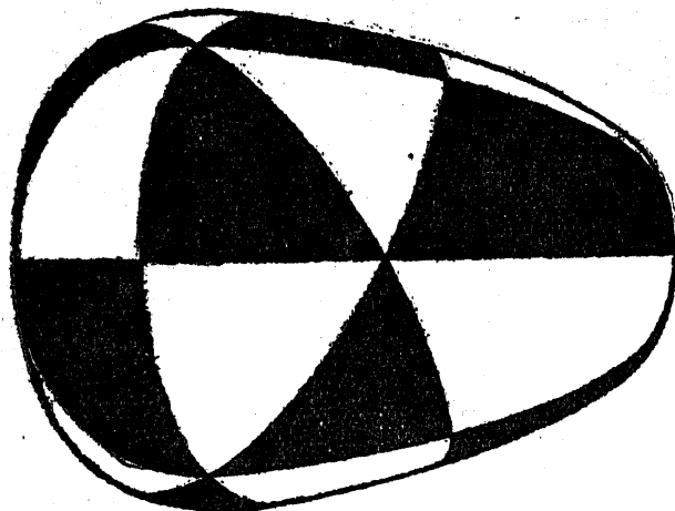
FIG. 6. Division of an ovaloid of revolution by the symmetry planes of a tetrahedron
