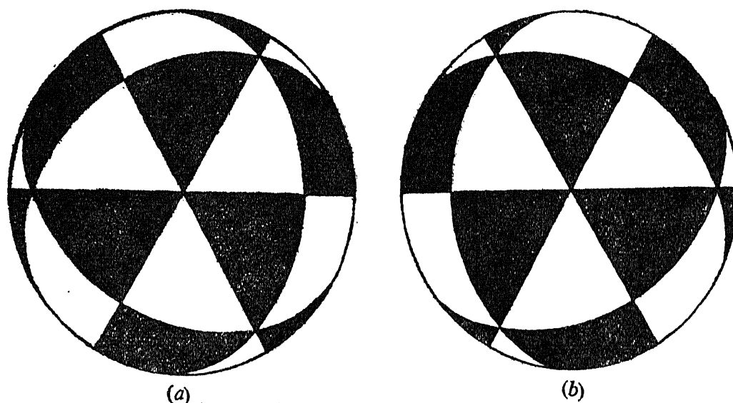
Figs. 5 (a) and (b). Division of an oblate spheroid by the symmetry planes of a tetrahedron
