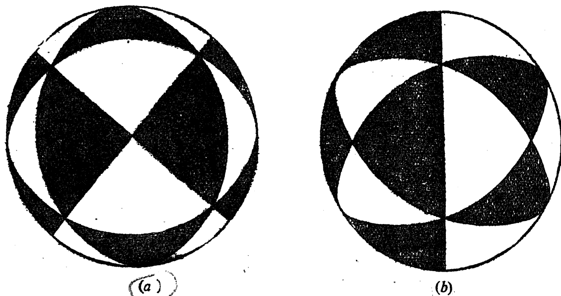
FIGS. 1 (a) and (b). Division of a spherical surface by the tetrahedral symmetry planes
