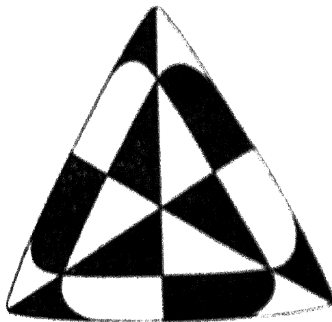
FIG. 11. Intersection of the tetrahedral symmetry planes with the two faces of a triangular twin.
