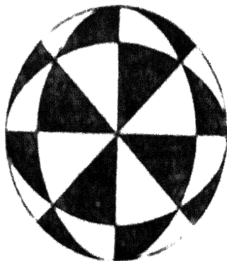
FIG. 3. Division of a spherical surface by the octahedral symmetry planes.
