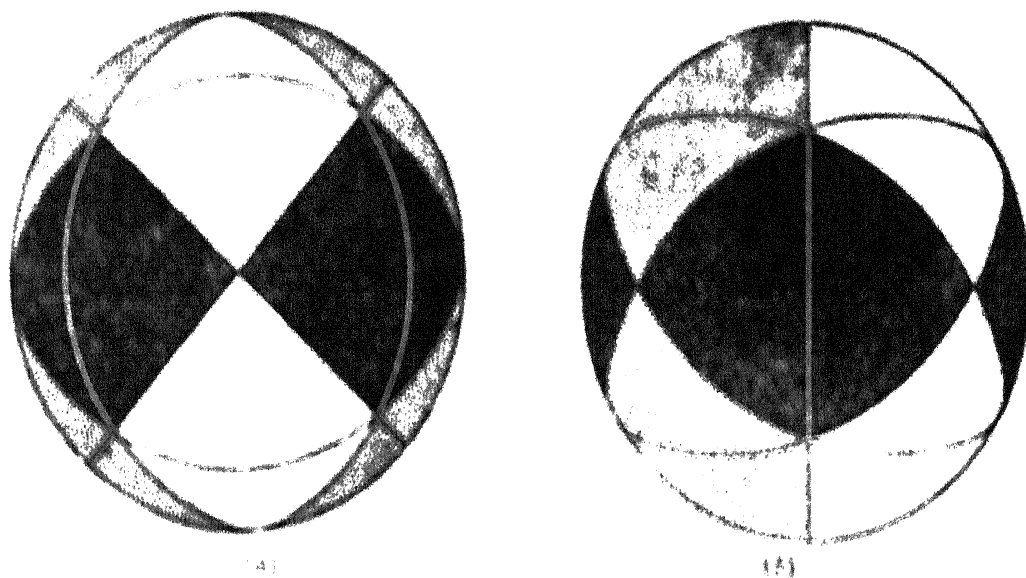
FIG. 2. (a) and (b). Rhombic dodecahedron projected on a sphere.
