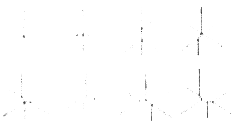
FIG. 8. Patterns of edges in the vicinity of a triad axis.
