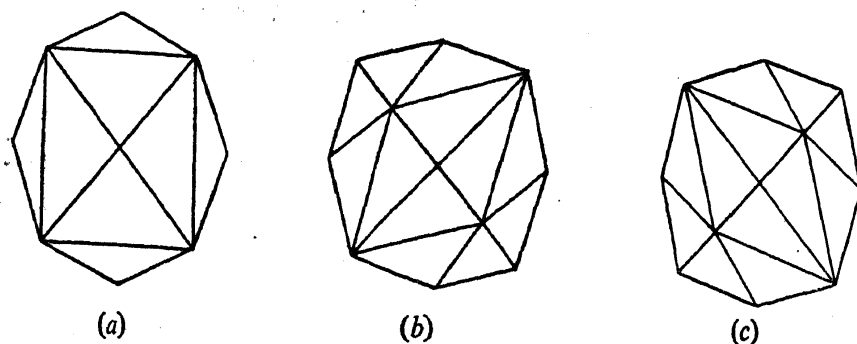
FIGS. 9 (a), (b) and (c). (a) Tetrakis-hexahedron; (b) and (c) Hexakis-tetrahedron viewed along a dyad axis
