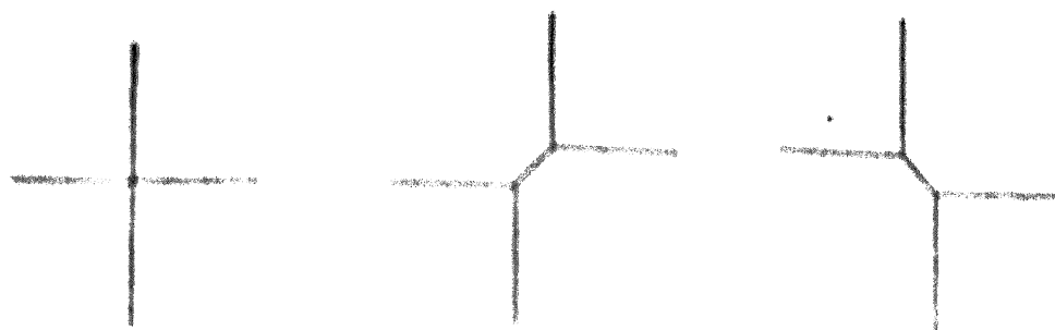
FIG. 7. Patterns of edges in the vicinity of a dyad axis.
