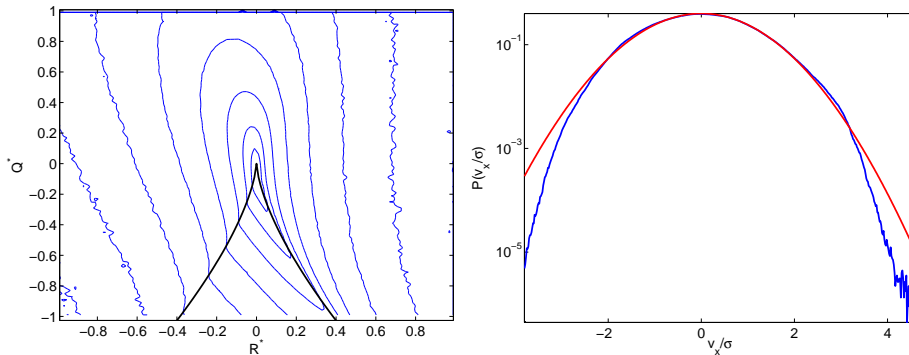
Figure 4. (Left) Joint PDF P(Q^*, R^*) of R^* = R/\langle s_{ij}s_{ij} \rangle^{3/2} and Q^* = Q/\langle s_{ij}s_{ij} \rangle calculated from our DNS. The black curve represents the zero-discriminant (or Vieillefosse) line 27R^2/4 + Q^3 = 0 . The contour levels are logarithmically spaced. (Right) PDF of the x -component of the velocity (here \sigma denotes the standard deviation); the parabolic curve is a Gaussian that is drawn for comparison.
