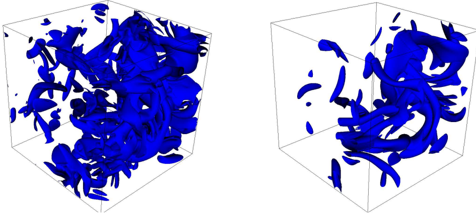
Figure 14. Constant- |\omega| isosurfaces for |\omega| = \langle |\omega| \rangle + \sigma at cascade completion without and (right) with polymers ( c = 0.4 ); \langle |\omega| \rangle is the mean and \sigma the standard deviation of |\omega| .
