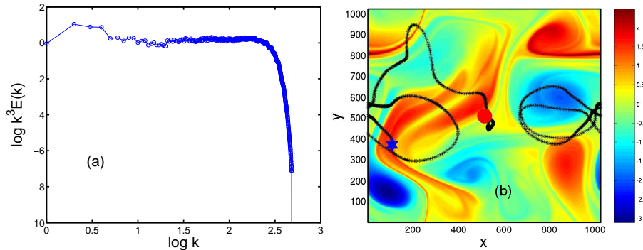
Figure 8. (a) A log–log plot of the compensated energy spectrum k^3 E(k) vs. k from our DNS, of resolution 1024^2 , of two-dimensional decaying turbulence with periodic boundary conditions. The flat region indicates a scaling form E(k) \sim k^{-3} . (b) The trajectory of a single Lagrangian particle over a time of order 100 in a two-dimensional flow with drag and forcing. The starting point of the trajectory is in the middle of the box and is indicated by a red circle; the end point is indicated by a blue star. The trajectory is superimposed on a pseudocolour plot of the vorticity field corresponding to the time at the end of the Lagrangian trajectory. The figure corresponds to a forced DNS of resolution 1024^2 with periodic boundary conditions, statistical steady state, and with a coefficient of Ekman friction \alpha_E = 0.1 .
