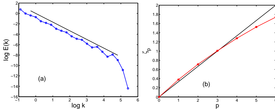
Figure 1. (a) A representative log–log plot of the energy spectrum E(k) vs. k , from a numerical simulation of the GOY shell model with 22 shells. The straight black line is a guide to the eye indicating K41 scaling k^{-5/3} . (b) A plot of the equal-time scaling exponent \zeta_p vs. p , with error bars, obtained from the GOY shell model. The straight black line indicates K41 scaling p/3 .
