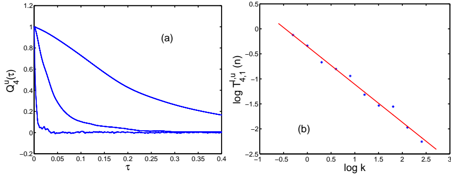
Figure 6. (a) A representative plot of the normalized fourth-order time-dependent structure function vs. the dimensionless time \tau obtained from the GOY shell model. The plots are for shells 4, 6, and 8 (from top to bottom). (b) A log–log plot of T_{4,1}^{I,u}(n) vs. k_n (for convenience, we have dropped the subscript n in the label of the x -axis in the figure); a linear fit gives the dynamic multiscaling exponent z_{4,1}^{I,u} .
