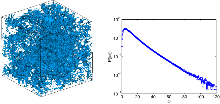
Figure 2. (Left) Isosurface plot of |\omega| with |\omega| equal to its mean value. (Right) A semilog plot of the PDF of |\omega| .
