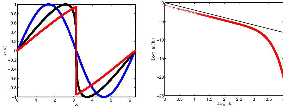
Figure 11. (Left) Snapshots of the solution of the Burgers equation obtained from our DNS with initial condition u(x) = \sin x at times t = 0 (blue), t = 1 (black) and t = 2 (red). (Right) A representative log–log plot of E(k) vs. k , at time t = 1 for the Burgers equation with initial conditions u(x) = \sin x .
