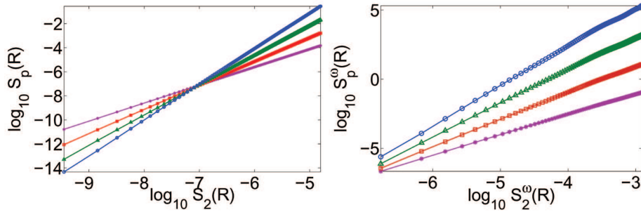
Figure 9. (Left) Log–log ESS plots of the isotropic parts of the order- p velocity structure functions S_p(R) vs. S_2(R) ; p = 3 (purple line with dots), p = 4 (red line with square), p = 5 (green line with triangles), and p = 6 (blue line with circles). According to the KLB prediction S_p(R) \sim R_p^\zeta . (Right) Log–log ESS plots of the isotropic parts of the order- p vorticity structure functions S_p(R) vs. S_2(R) ; p = 3 (purple line with stars), p = 4 (red line with square), p = 5 (green line with triangles), and p = 6 (blue line with circles).
