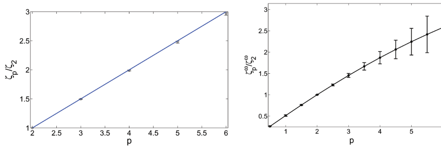
Figure 10. (Left) Plots of the exponent ratios \zeta_p/\zeta_2 vs. p for the velocity differences. (Right) Plots of the exponent ratios \zeta_p^\omega/\zeta_2^\omega vs. p for the vorticity differences.
