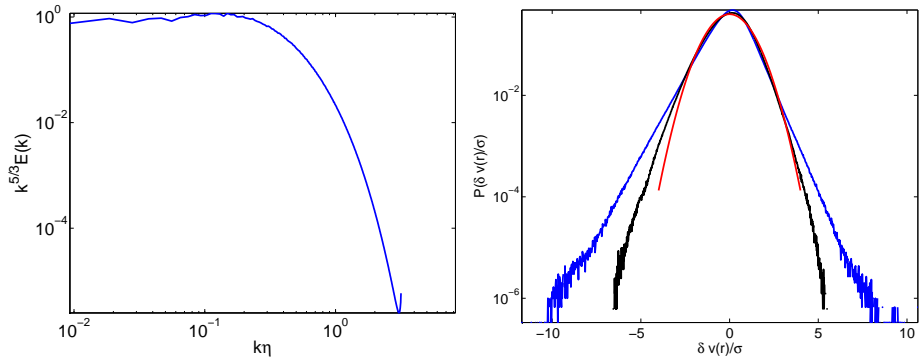
Figure 5. (Left) The compensated energy spectrum k^{5/3}E(k) vs. k\eta , where \eta is the dissipation scale from our DNS (see text). (Right) PDFs of velocity increments that show marked deviation from Gaussian behaviour (innermost curve), especially at small length scales; the outermost PDF is for the velocity increment with the shorter length scale.
