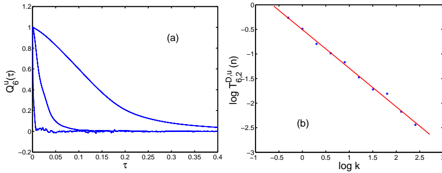
Figure 7. (a) A representative plot of the normalized sixth-order time-dependent structure function vs. the dimensionless time \tau obtained from the GOY shell model. The plots are for shells 4, 6, and 8 (from top to bottom). (b) A log–log plot of T_{6,2}^{D,u}(n) vs. k_n (for convenience, we have dropped the subscript n in the label of the x -axis in the figure); a linear fit gives the dynamic multiscaling exponent z_{6,2}^{D,u} .
