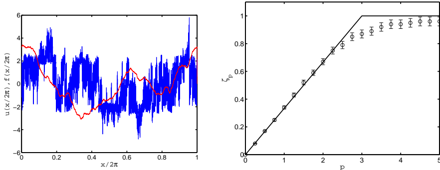
Figure 12. (Left) A snapshot of the velocity field (jagged line in blue) in steady state and the force in red from our fast Legendre method DNS of the stochastically forced Burgers equation. (Right) A representative plot of the exponents \zeta_p , with error bars, for the equal time velocity structure functions of the stochastically forced Burgers equation. Bifractal scaling is shown by the black solid line and the deviations from this are believed to arise from artefacts (see text).
