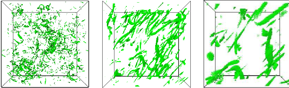
Figure 3. (Left) Isosurface plot of |\omega| with |\omega| equal to one standard deviation more than its mean value. (Centre) A magnified version of the central part of the panel on the left. (Right) A magnified version of the central part of the panel in the middle.
