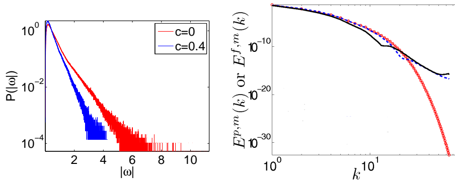
Figure 15. (Left) PDF of \omega at cascade completion without ( c = 0 ) and with polymers ( c = 0.4 ). Note that regions of large vorticity are reduced on the addition of polymers. (Right) Representative plots of the energy spectra E^{p,m}(k) or E^{f,m}(k) vs. k for c = 0.1 (blue dashed line) and c = 0.4 (solid line).
