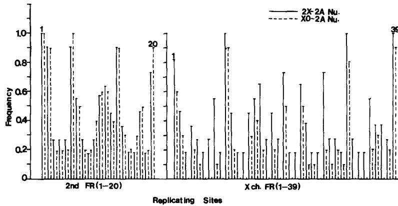
FIGURE 7 Histograms showing the frequencies of [^3\text{H}]\text{TdR} labeling of the 20 replicating units of the 2R segment and the 39 replicating units of the X chromosome segment of the XX2A (female) and XO2A (male) nuclei in the mosaic salivary glands of D. melanogaster .
