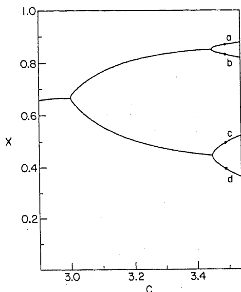
Figure 2. Lower period branches of the bifurcation diagram for the single logistic map.
