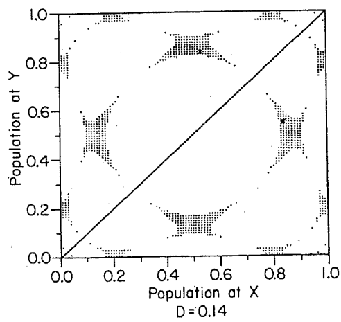
Figure 3(a)-(c). Shrinking basin of attraction for a period-2 flip-flop cycle as D is increased, with c = 3.625 . Points on the limit cycle are denoted by x .
