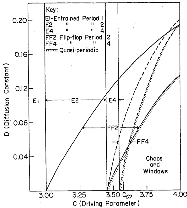
Figure 1. Parameter space diagram showing the stability regions of the lower period-2 n entrained and flip-flop cycles.
