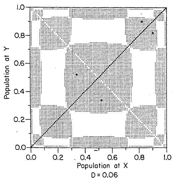
Figure 3(d). Basin of attraction for a period-4 flip-flop cycle for c = 3.625 and D = 0.06 . Points on the limit cycle are denoted by 0.
