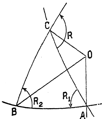
FIG. 1. Composition of Rotations: 2R_1 + 2R_2 = 2R .
