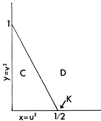
FIG. 4. Phase diagram in the (x,y) plane. The transition is Kasteleyn or commensurate-incommensurate type for y=0 , for which dislocations are not allowed, and Ising type for y \neq 0 , for which dislocations are allowed. The point K = (\frac{1}{2}, 0) is the multicritical point, called the Kasteleyn point. C represents the commensurate phase and D the disordered phase.
