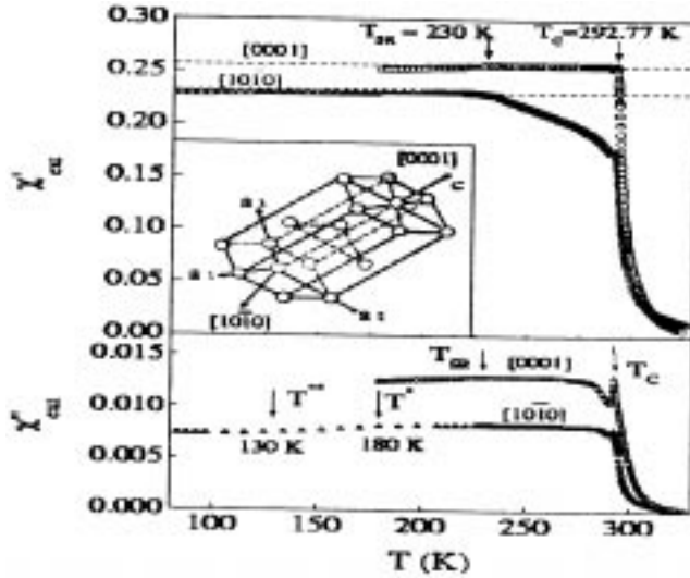
Figure 4. Temperature dependence of the real ( \chi'_{\text{ext}} ) and imaginary ( \chi''_{\text{ext}} ) components of ac susceptibility of single crystal sample 2 of Gd at 87 Hz frequency for ac field amplitude of 10 mOe applied along the crystallographic directions [0001] (open circles) and [10 \bar{1} 0] (open triangles) (ref. [15]). The inset shows the crystal structure of Gd indicating the directions [0001] and [10 \bar{1} 0]. The horizontal dashed lines indicate the demagnetisation limited value \chi'_{\text{ext}} = 1/4\pi N_d (see text).
