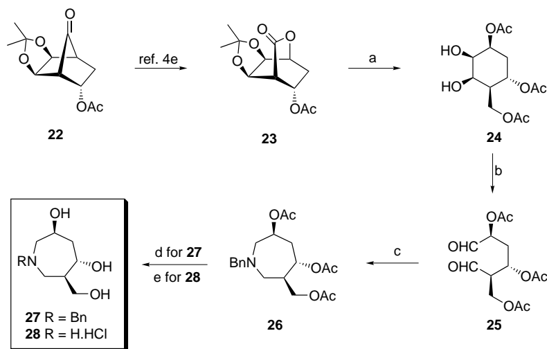
Scheme 3. Reagents and conditions: (a) i. LAH, THF, 0–5°C, 3 h, 70%, ii. Ac 2 O, DMAP, DCM, rt, 12 h, 89%, iii. Amberlyst-15, THF–H 2 O (2:3), rt, 12 h, 85%; (b) NaIO 4 –silica gel, DCM, 0°C, 2 h; (c) BnNH 2 , AcOH, NaCNBH 3 , MeOH, 15 h, 30% (two steps); (d) K 2 CO 3 , MeOH, rt, 6 h, quant.; (e) i. H 2 , Pd/C, EtOH, rt, 5 h, ii. 1N HCl, 90°C, 20 h, 90%.
