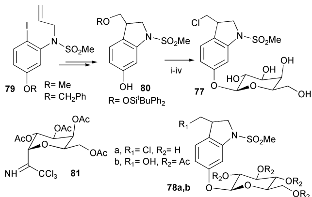
Scheme 16 Reagents and conditions: i, 81 , \text{BF}_3 \cdot \text{OEt}_2 , molecular sieves; ii, TBAF, \text{SiO}_2 ; iii, \text{PPh}_3 , \text{CCl}_4 ; iv, \text{K}_2\text{CO}_3 , MeOH.
