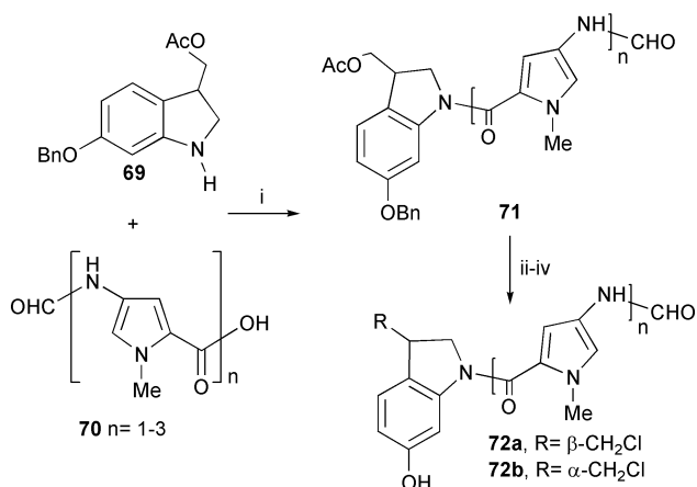
Scheme 14 Reagents and conditions: i, \text{EDCI} \cdot \text{HCl} ; ii, \text{LiOH} \cdot \text{H}_2\text{O} ; iii, \text{Ph}_3\text{P} , \text{CCl}_4 ; iv, \text{BBr}_3 .
