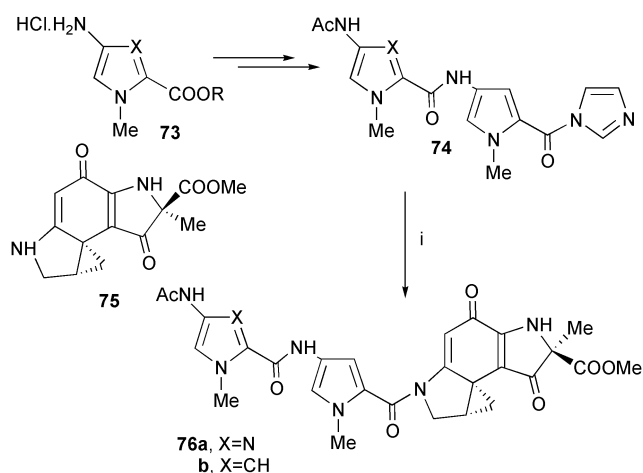
Scheme 15 Reagents and conditions: i, 75 , NaH, DMF, ( X = \text{N} , 38%; X = \text{CH} , 26%).
