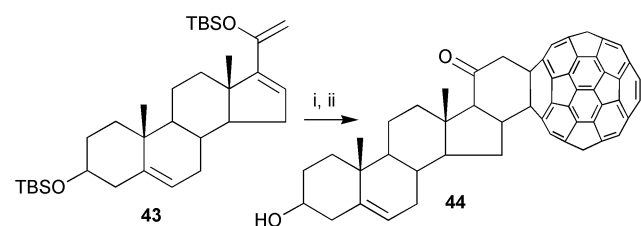
Scheme 10 Reagents and conditions: i, C 60 , Δ; ii, p -TsOH, Δ.
