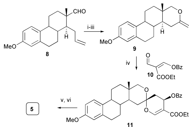
Scheme 1 Reagents and conditions: i, \text{NaBH}_4 ; ii, \text{I}_2 , \text{NaHCO}_3 ; iii, DBU; iv, 10 ; v, DIBAH; vi, \text{PtO}_2 , \text{H}_2 , 50 bar.
