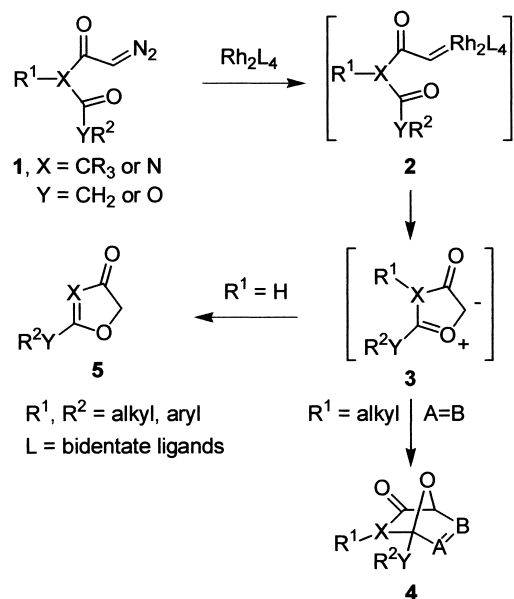
Scheme 1.
