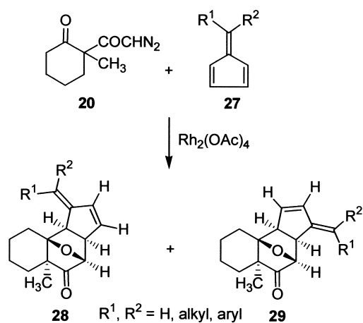
Scheme 8.
