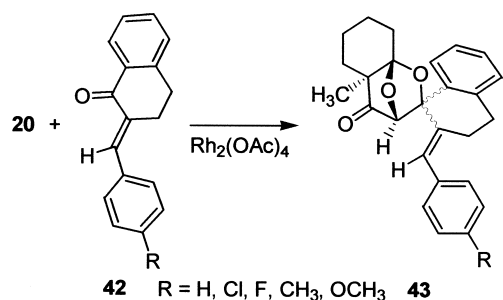
Scheme 13.
