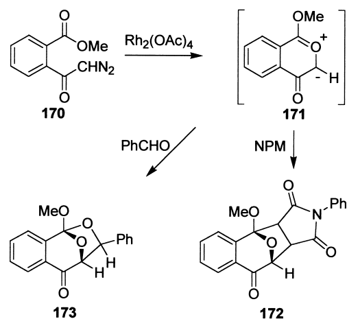
Scheme 51.
