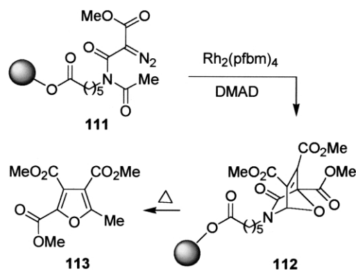
Scheme 32.
