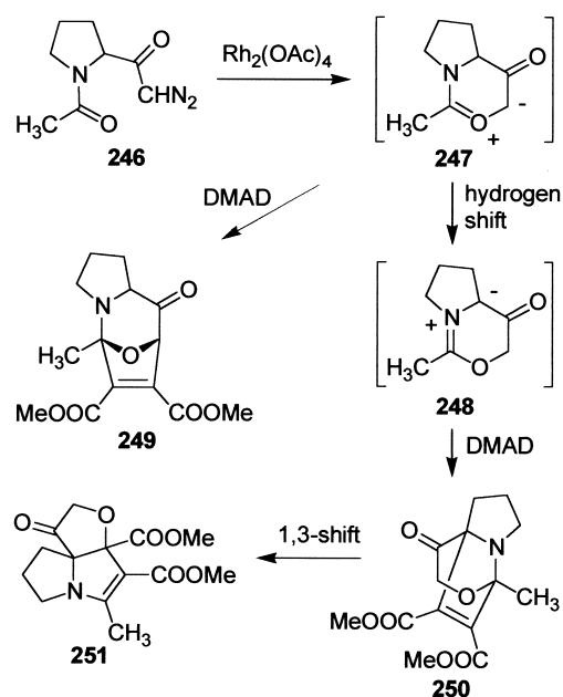
Scheme 77.
