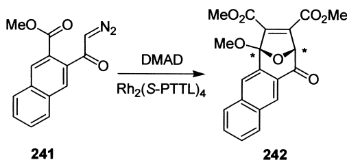
Scheme 75.
