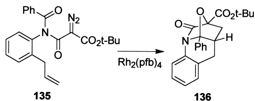
Scheme 40.
