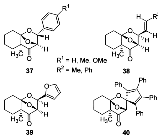
Scheme 11.
