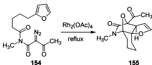
Scheme 46.
