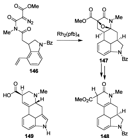
Scheme 44.
