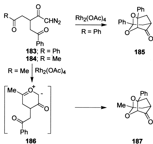
Scheme 56.
