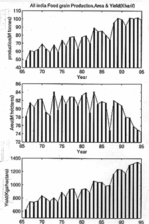
Figure 5. All India foodgrain production in m tons (top); area in million hectares (middle); yield in kg/hectare (bottom) for kharif season. Source: Same as Figure 1.
