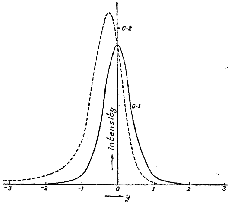
FIG. 3. Reflection (full line) and Transmission (dotted line) Curves of a crystal of calcite 0.4 mm. thick. y = 1 corresponds to 3.6'' of arc.
