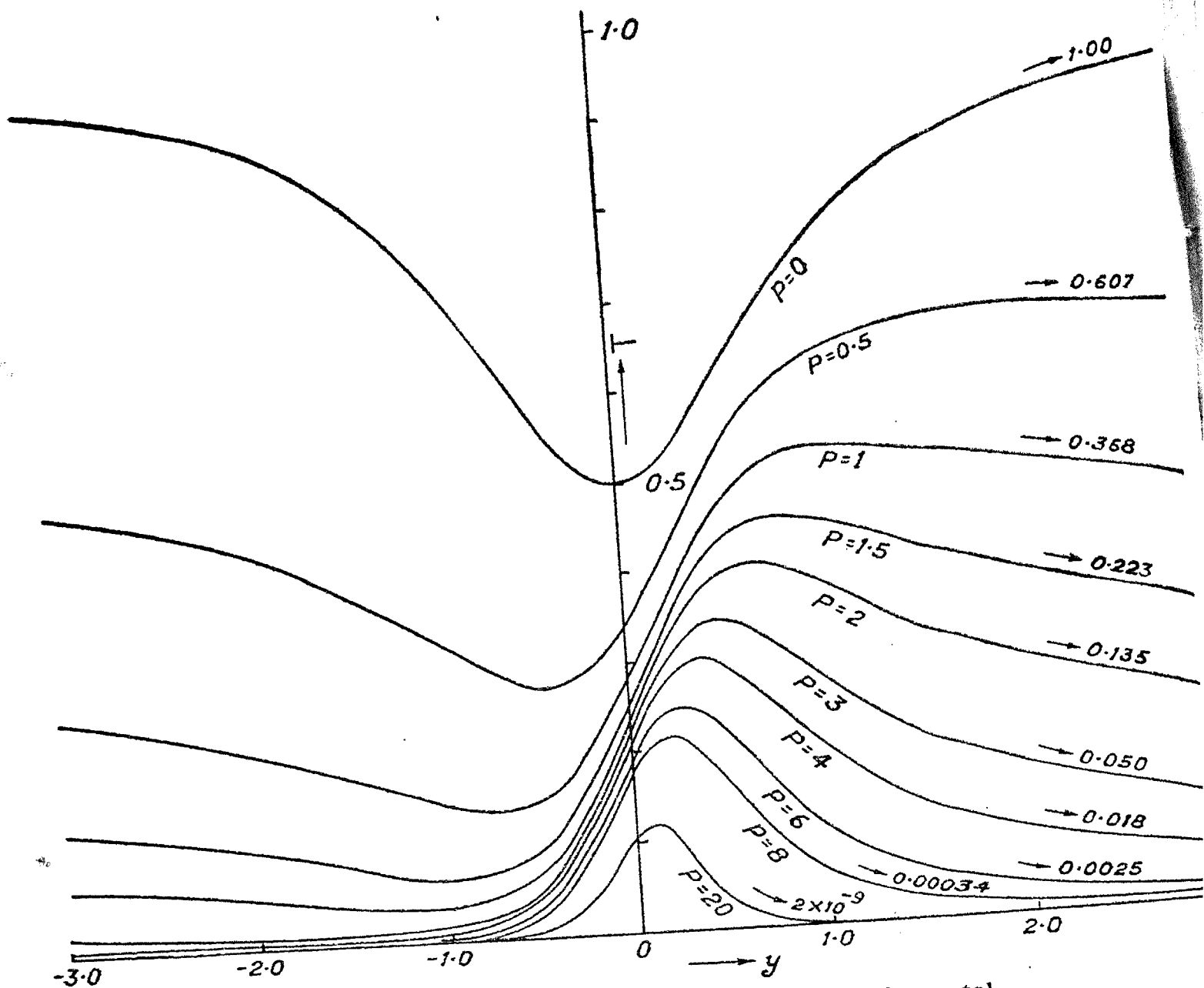
FIG. 2. Transmission curves for varying thickness of the crystal.
