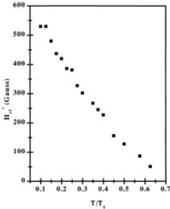
Figure 3. H_{c1}^* obtained from the slope change observed in the NRMA signals from MgB_2 uncorrected for demagnetization factor and geometrical and/or surface barrier effects, plotted as a function of reduced temperature ( T/T_c ), showing quasi-linear behavior.
