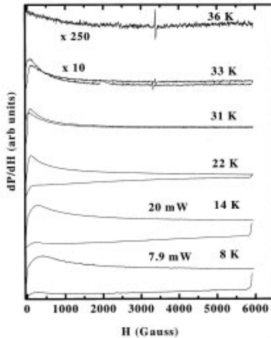
Figure 2. Typical NRMA signals from a sample of MgB_2 + MgO recorded during warming at a few representative temperatures for both forward and reverse scans of the magnetic field. The signals show strong zero field response indicating the presence of weak links acting as JJs. The hysteresis between forward and reverse scans of the magnetic field shows a strong field as well as temperature dependence.
