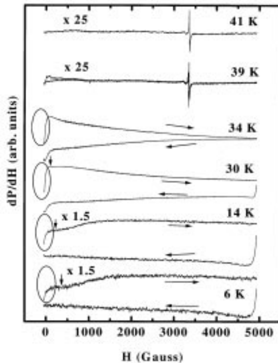
Figure 1. Typical NRMA signals recorded from a sample of \text{MgB}_2 during warming at a few representative temperatures for both forward and reverse scans of the magnetic field. The ellipses indicate part of the signal tentatively attributed to a very small number of weak links forming JJs in the sample. The vertical arrows mark the field at which the slope changes indicating the onset of the entry of the magnetic field in the form of vortices in the sample. The hysteresis between the forward and reverse scans of the magnetic field shows near field independence, thus forming practically rectangular hysteresis loop.
