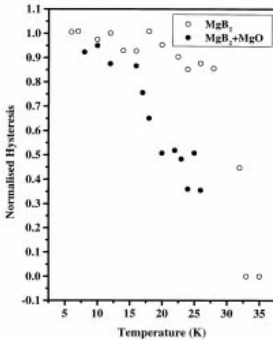
Figure 4. The ratio of hysteresees at 4000 Gauss to 2000 Gauss plotted as a function of temperature for the samples of \text{MgB}_2 and \text{MgB}_2 + \text{MgO} . In the case of pure \text{MgB}_2 (open circles), the ratio of \sim 1 independent of temperature till about 27 K indicates a very strong pinning of flux lines. In the case of \text{MgB}_2 + \text{MgO} (solid circles) the ratio is strongly temperature dependent and is less than unity in most of the temperature range indicating weaker pinning.
