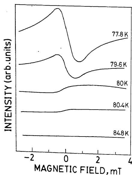
Figure 1. Near-zero-field signal of \text{YBa}_2\text{Cu}_3\text{O}_{7-x} as a function of temperature in the superconducting state.
