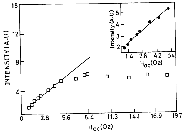
Figure 4. Intensity of the derivative signal as a function of the modulation amplitude for the film marked B in table 1. The inset shows the region of the linear fit expanded.
