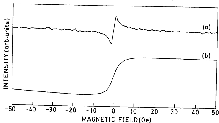
Figure 5. Field derivative of the non-resonant absorption signals for the YBCO thin film at (a) 19.5 MHz and (b) 9.1 GHz. To be noted is the drastic difference in the lineshapes at the two frequencies.
