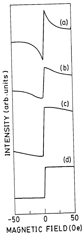
Figure 7. Simulation of the field derivative of the non-resonant absorption signals for different values of B_0 : (a) 10 Oe, (b) 30.3 Oe, (c) 100 Oe and (d) 1000 Oe.
