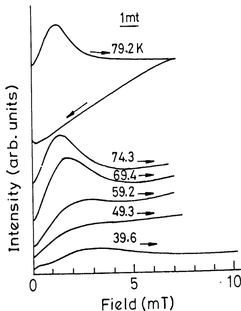
Figure 2. Derivative signals recorded at 13.35 MHz at different temperatures with a CW NMR spectrometer.
