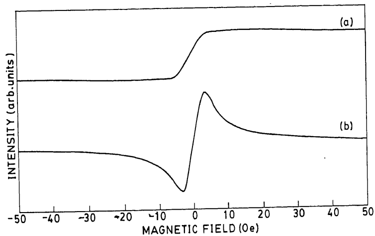
Figure 6. Field derivative of the non-resonant microwave absorption signal ( \omega = 9.1 GHz) for (a) the YBCO thin film and (b) the YBCO pellet.
