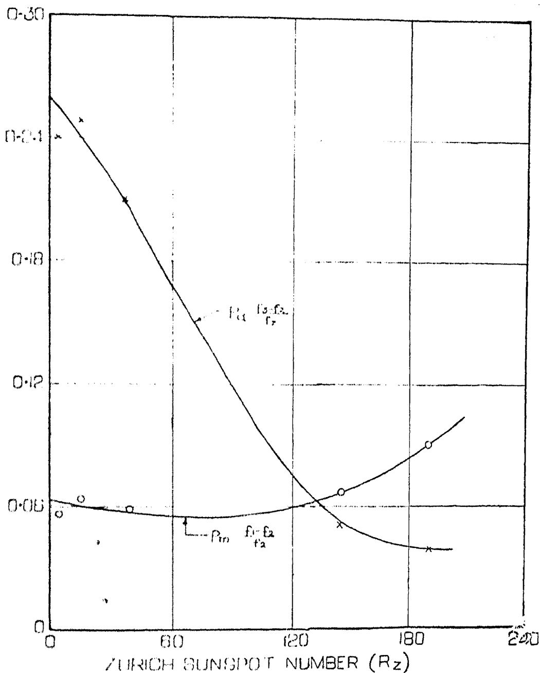
FIG. 8. Comparative Behaviour of Morning and Afternoon Peaks with Sunspot Activity.
