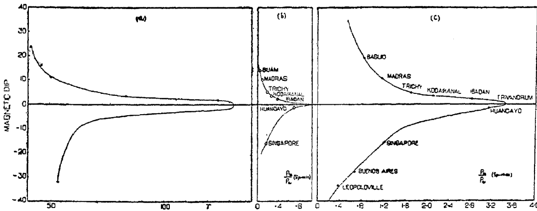
FIG. 7. (a) Distribution of Ranges of Daily Variation of the Horizontal Force against Magnetic Dip (After J. Egedal). (b) Variation of P_m/P_a with Magnetic Dip (Sp-min.). (c) Variation of P_m/P_a with Magnetic Dip (Sp-max.).
