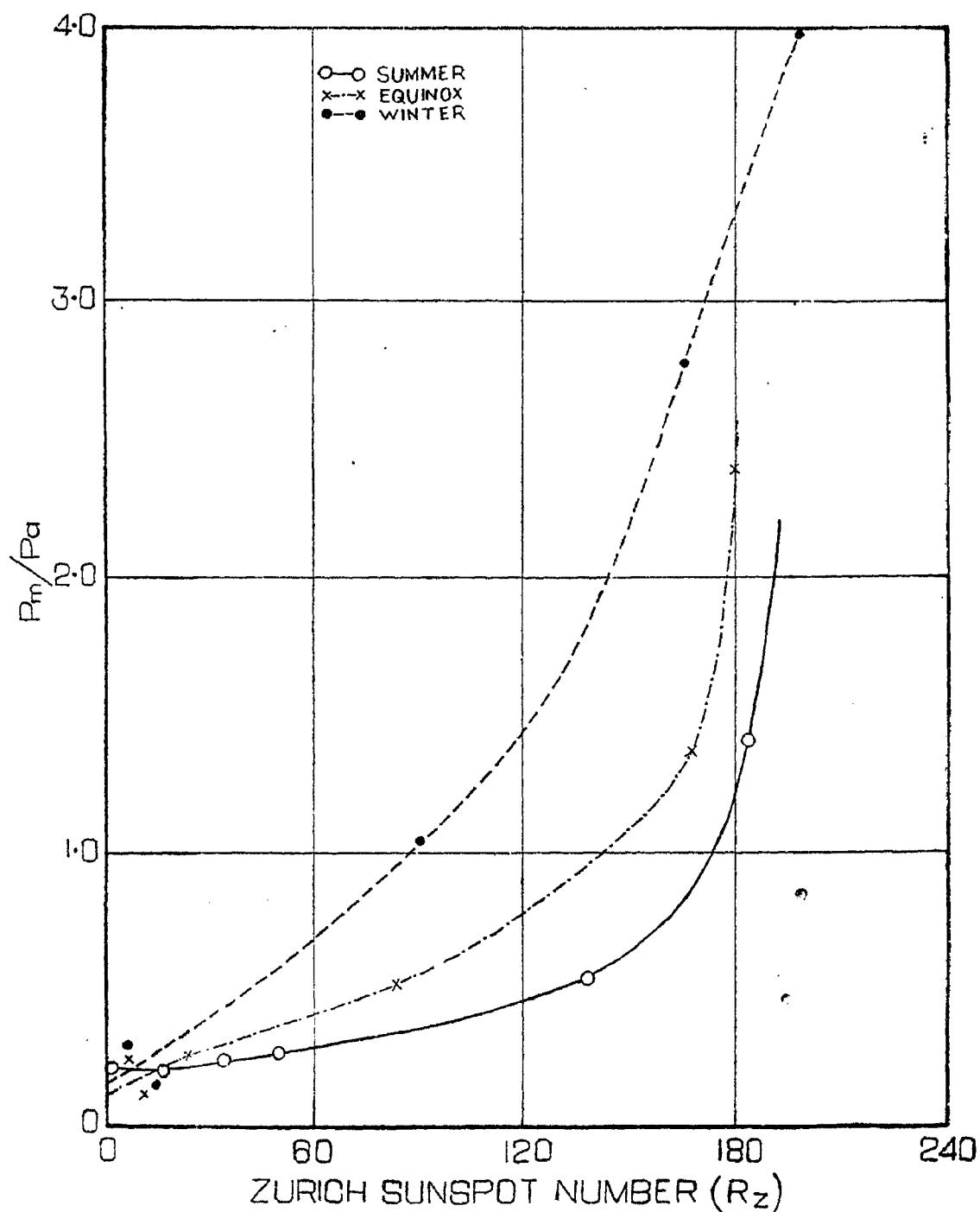
FIG. 6. Variation of P_m/P_a with Sunspot Activity for the Three Seasons.
