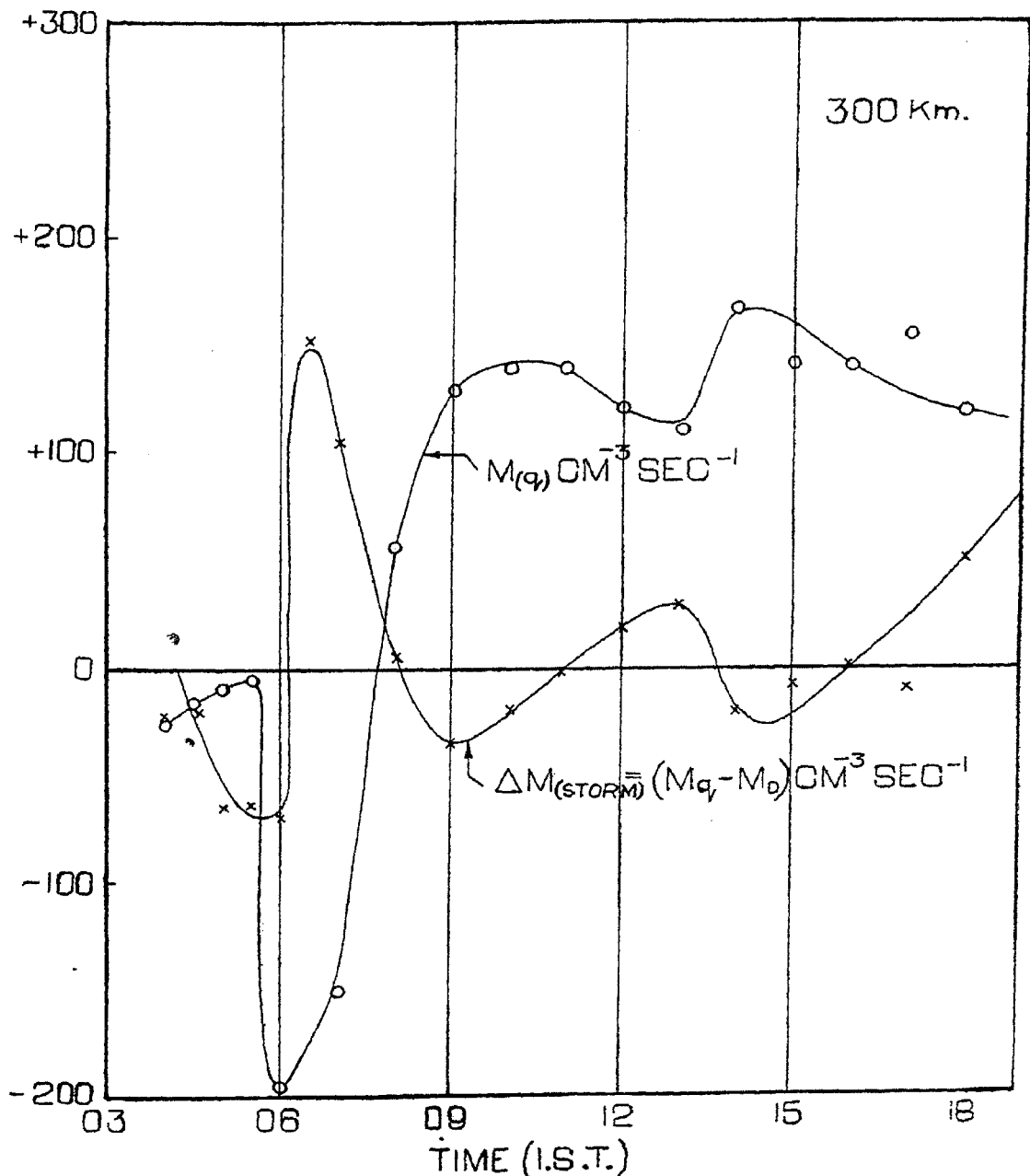
FIG. 4. Variation of Movement Term M (Quiet) = (N \cdot dw/dh) \text{ cm}^{-3} \cdot \text{sec}^{-1} with time together with \Delta M (due to storm). For 300 km. level.
