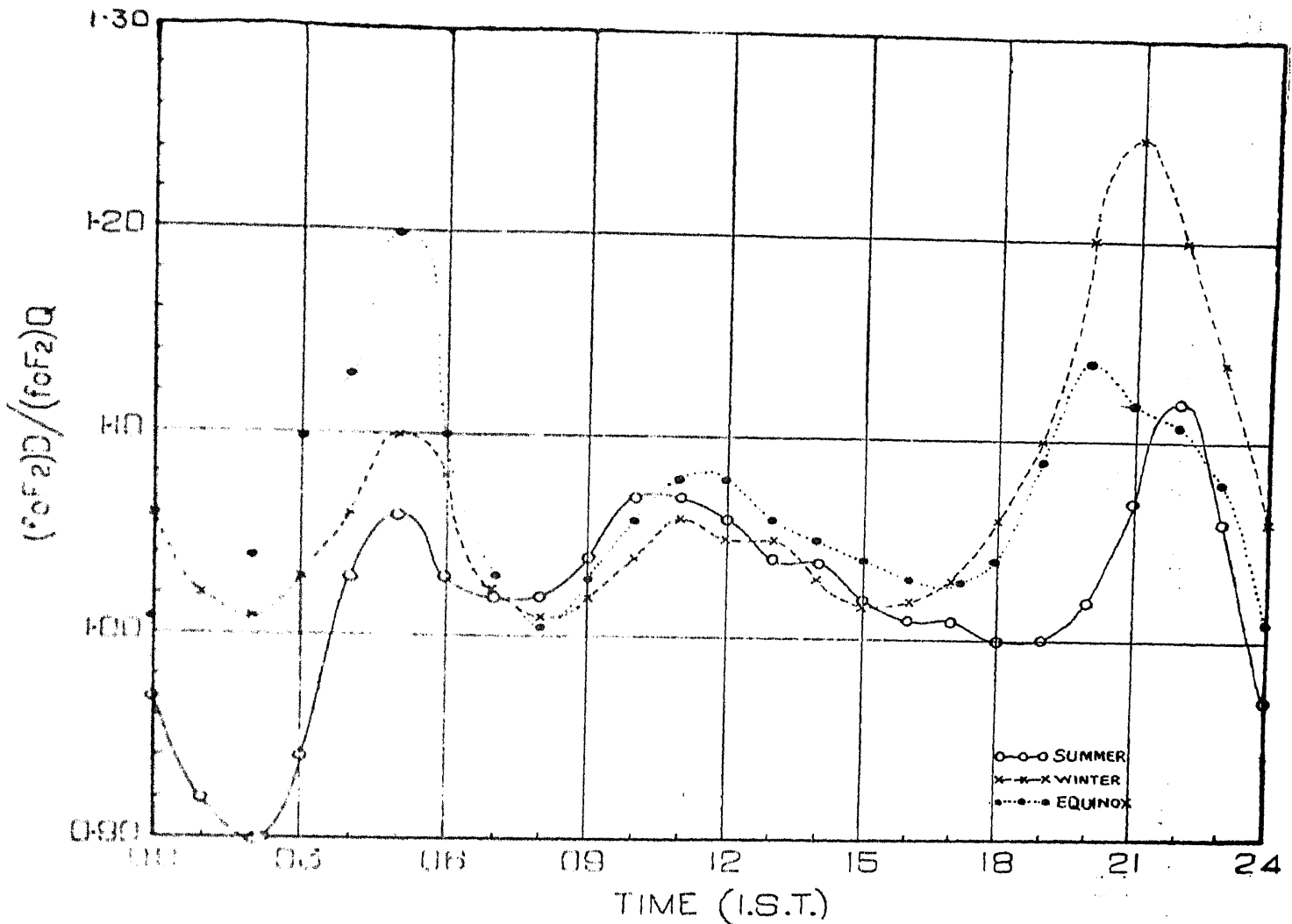
FIG. 2. Curve showing Diurnal Course of D(foF2)/Q(foF2) for three seasons.
